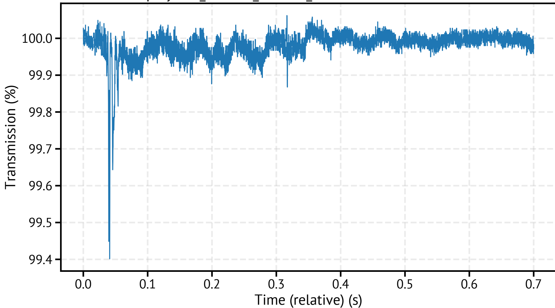
spraytec5_260318_112328_349400.csv - Transmission
