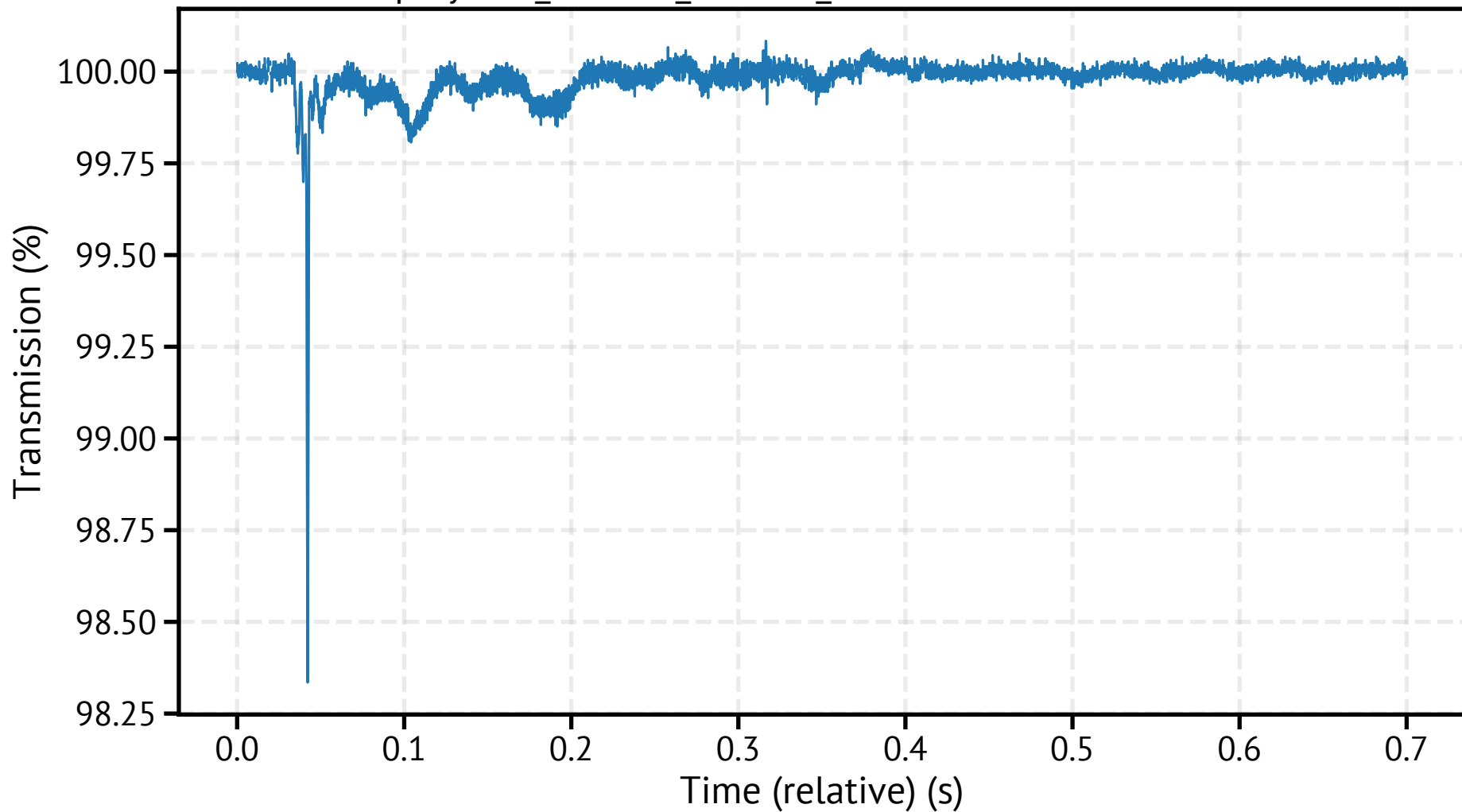
spraytec6_260318_112426_063900.csv - Transmission
