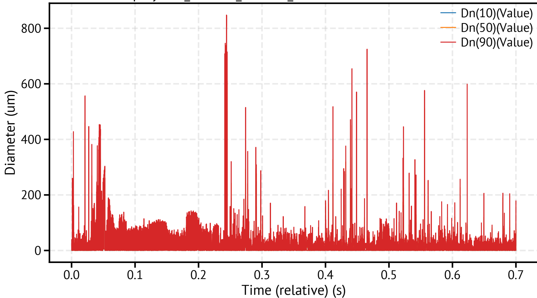
spraytec8_260318_112621_348200.csv - Dn Percentiles
