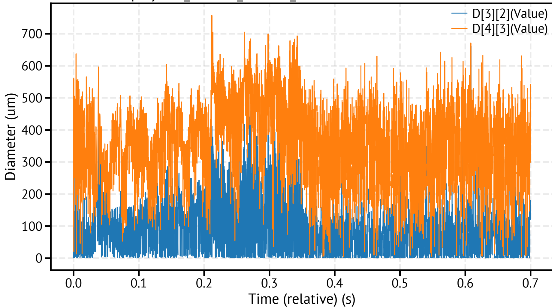
spraytec4_260318_113641_965300.csv - Mean Diameters
