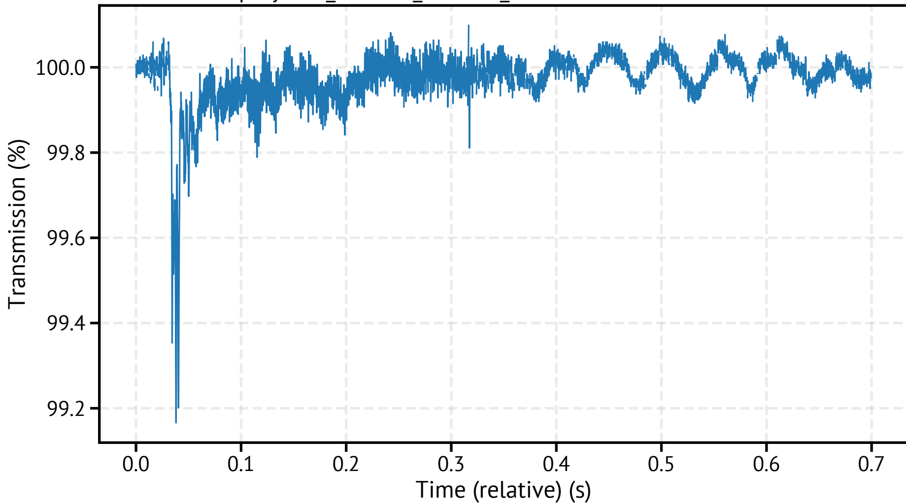
spraytec4_260318_113641_965300.csv - Transmission
