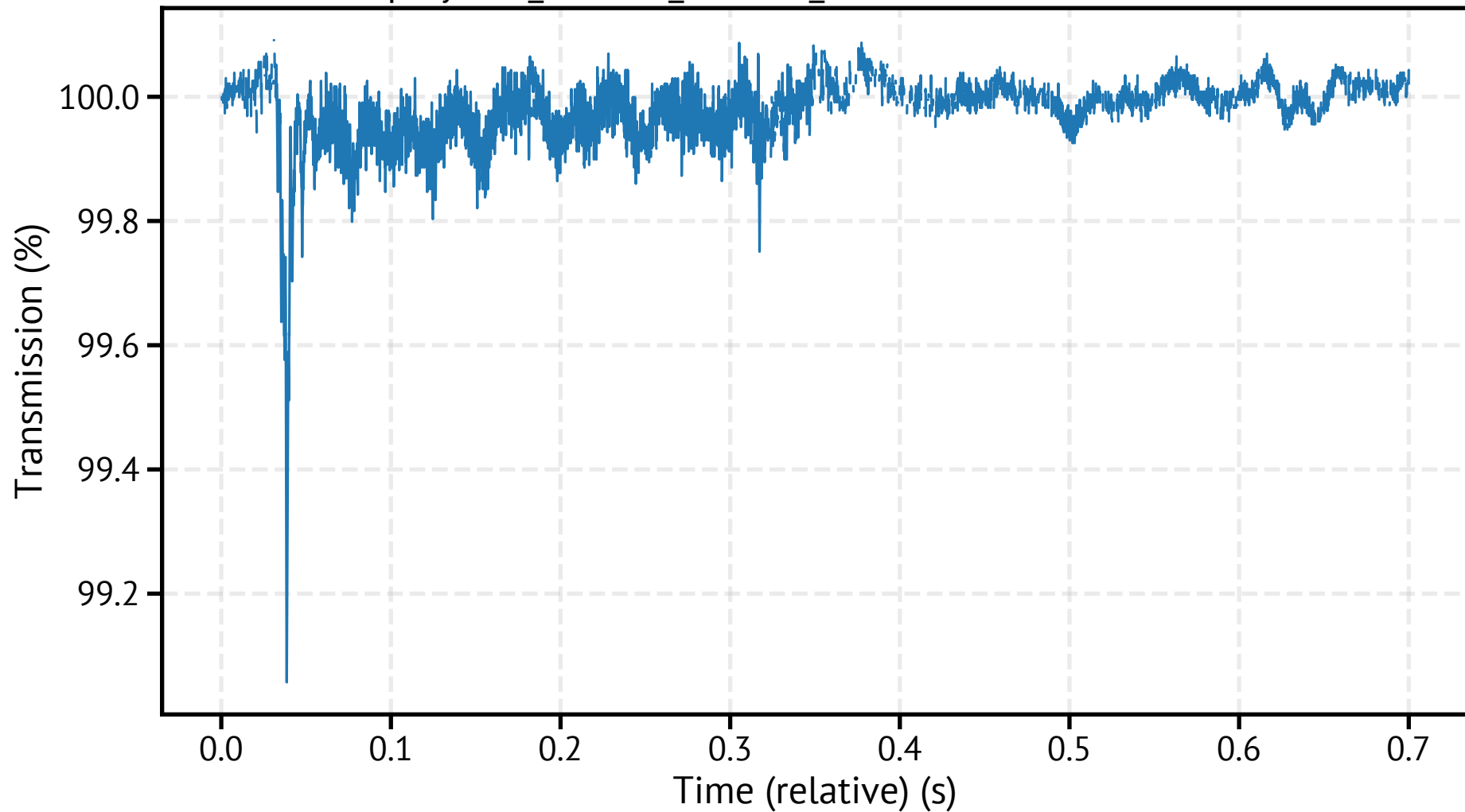
spraytec6_260318_113837_249900.csv - Transmission
