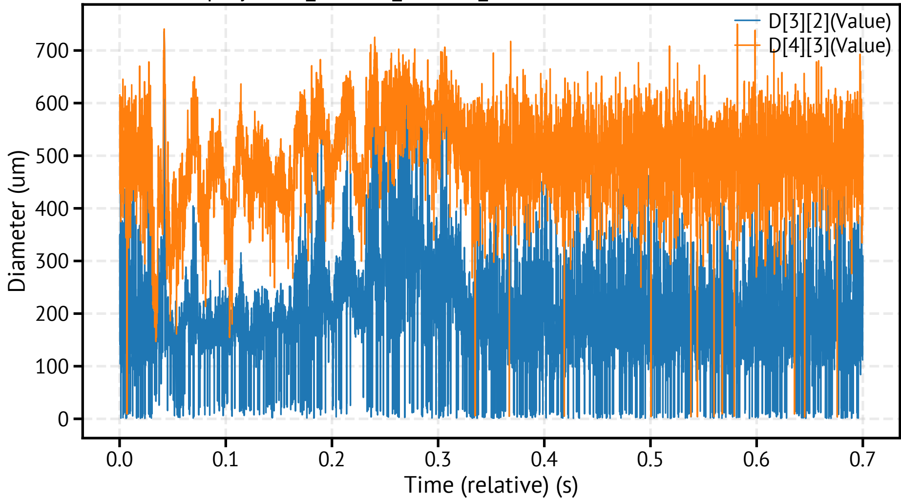
spraytec10_260318_115732_937600.csv - Mean Diameters
