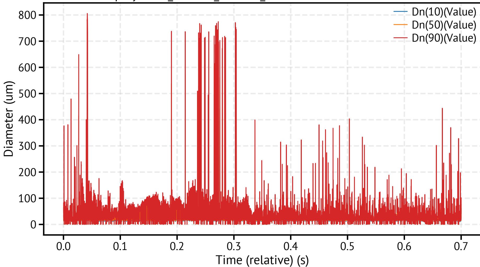
spraytec10_260318_115732_937600.csv - Dn Percentiles
