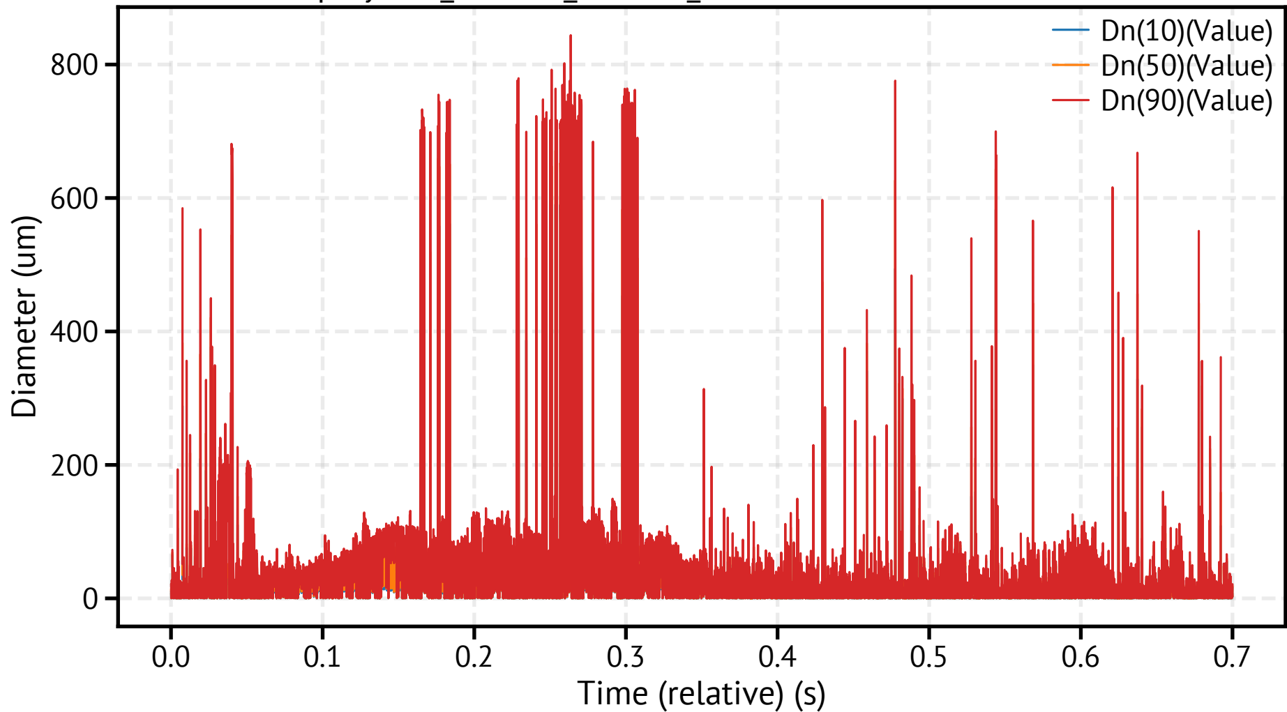
spraytec1_260318_114854_051000.csv - Dn Percentiles
