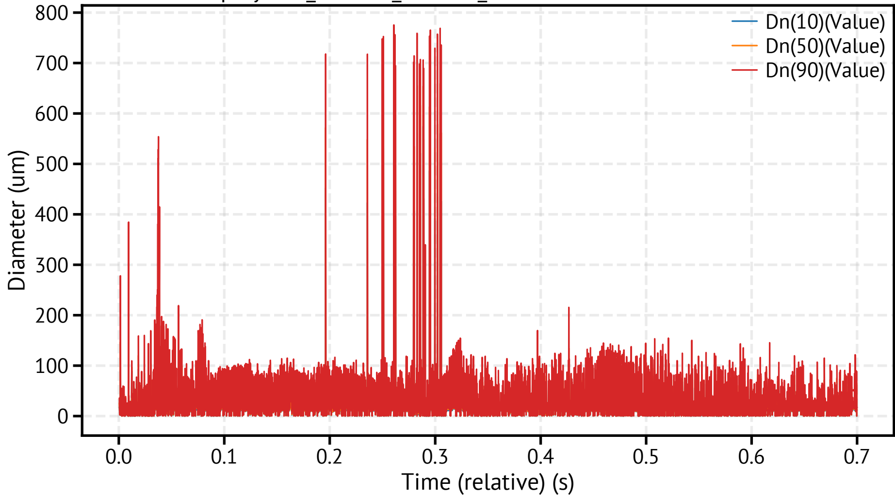
spraytec2_260318_114951_739900.csv - Dn Percentiles
