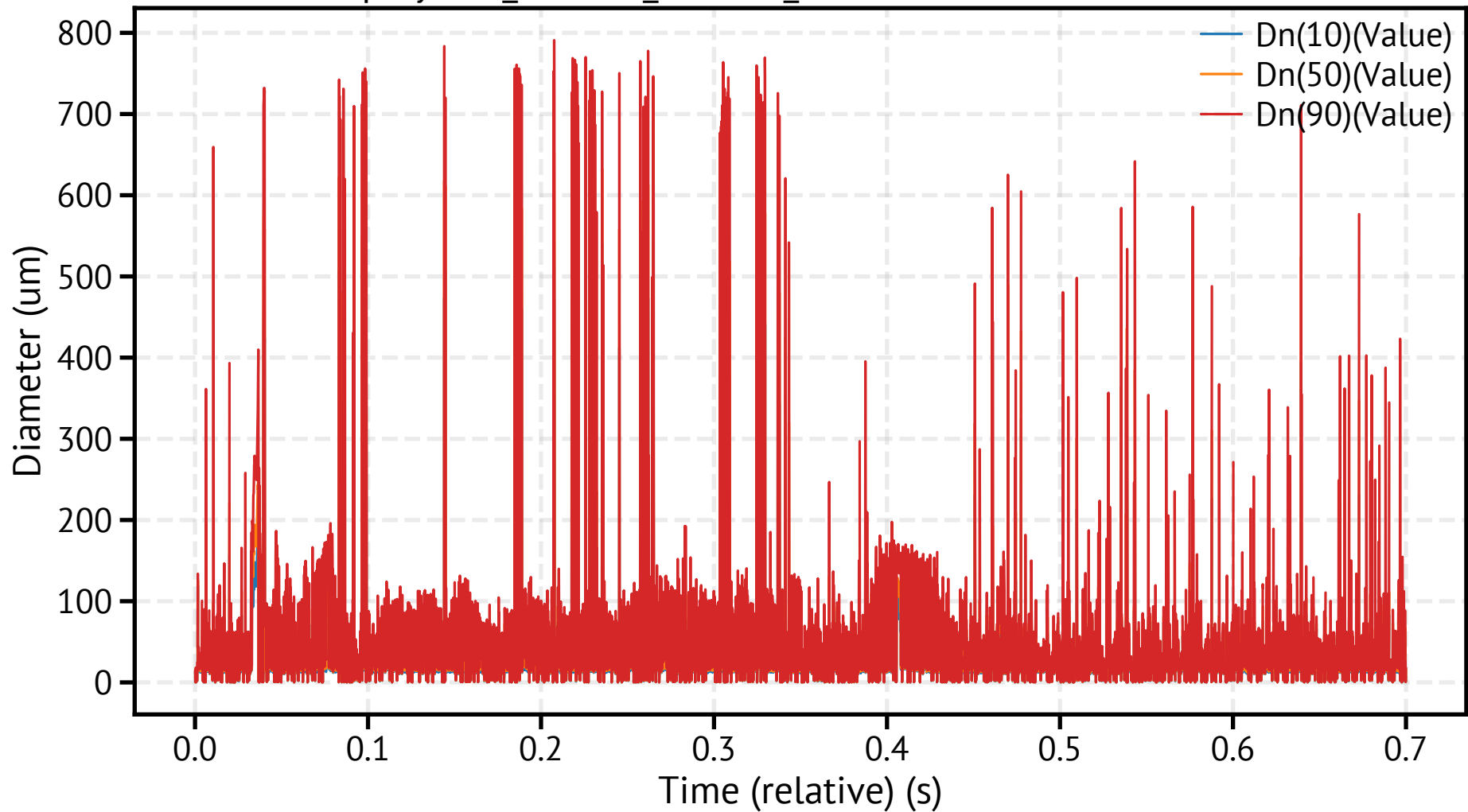
spraytec5_260318_115244_685800.csv - Dn Percentiles
