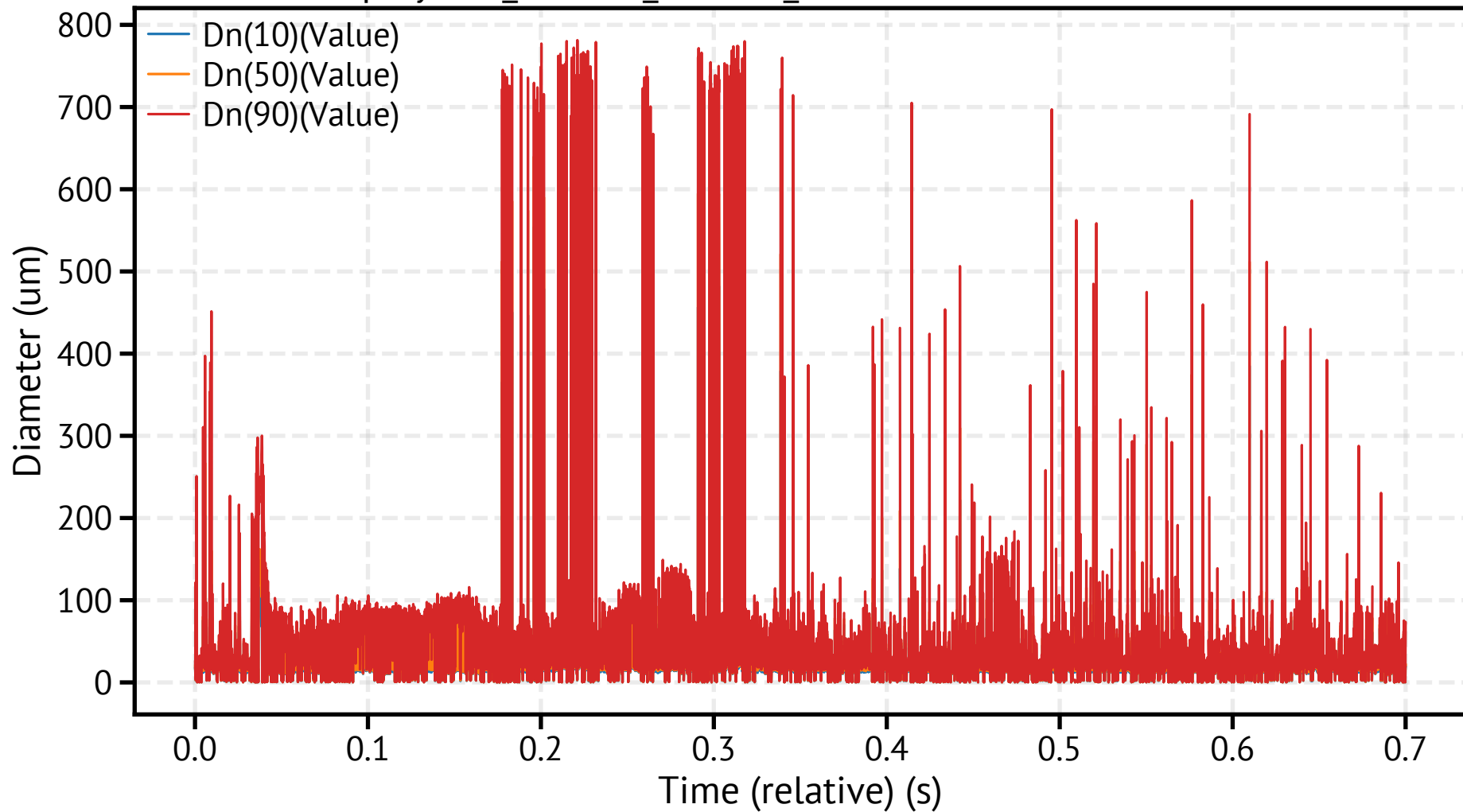
spraytec6_260318_115342_353900.csv - Dn Percentiles
