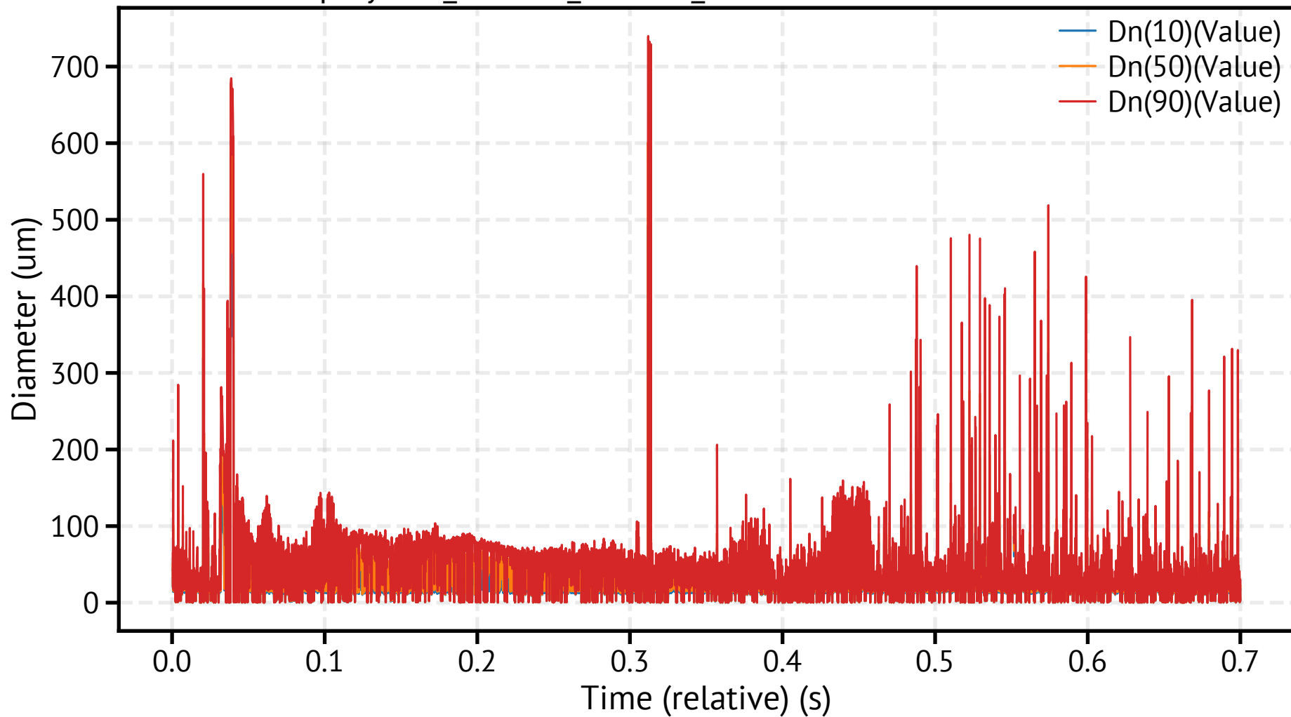
spraytec7_260318_115440_025200.csv - Dn Percentiles
