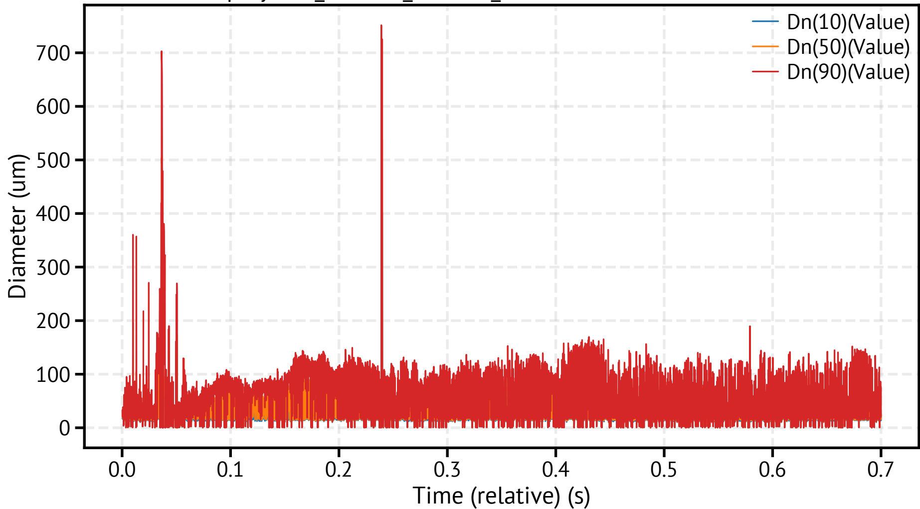
spraytec8_260318_115537_667200.csv - Dn Percentiles
