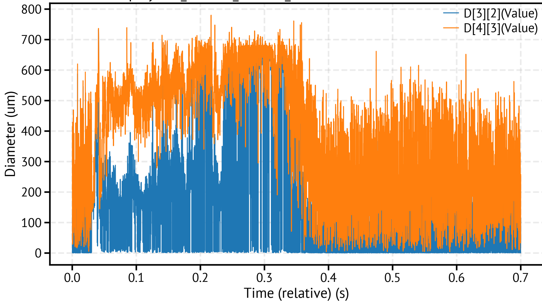
spraytec1_260318_120750_309000.csv - Mean Diameters
