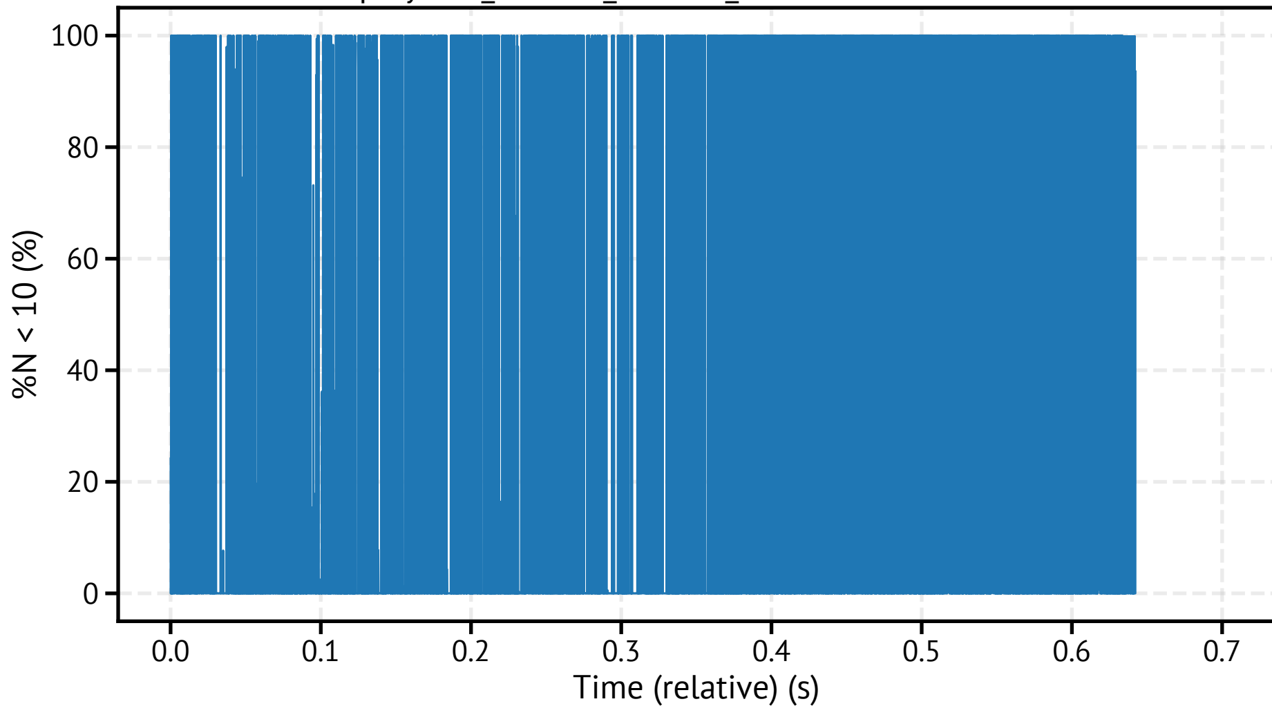
spraytec1_260318_120750_309000.csv - %N < 10
