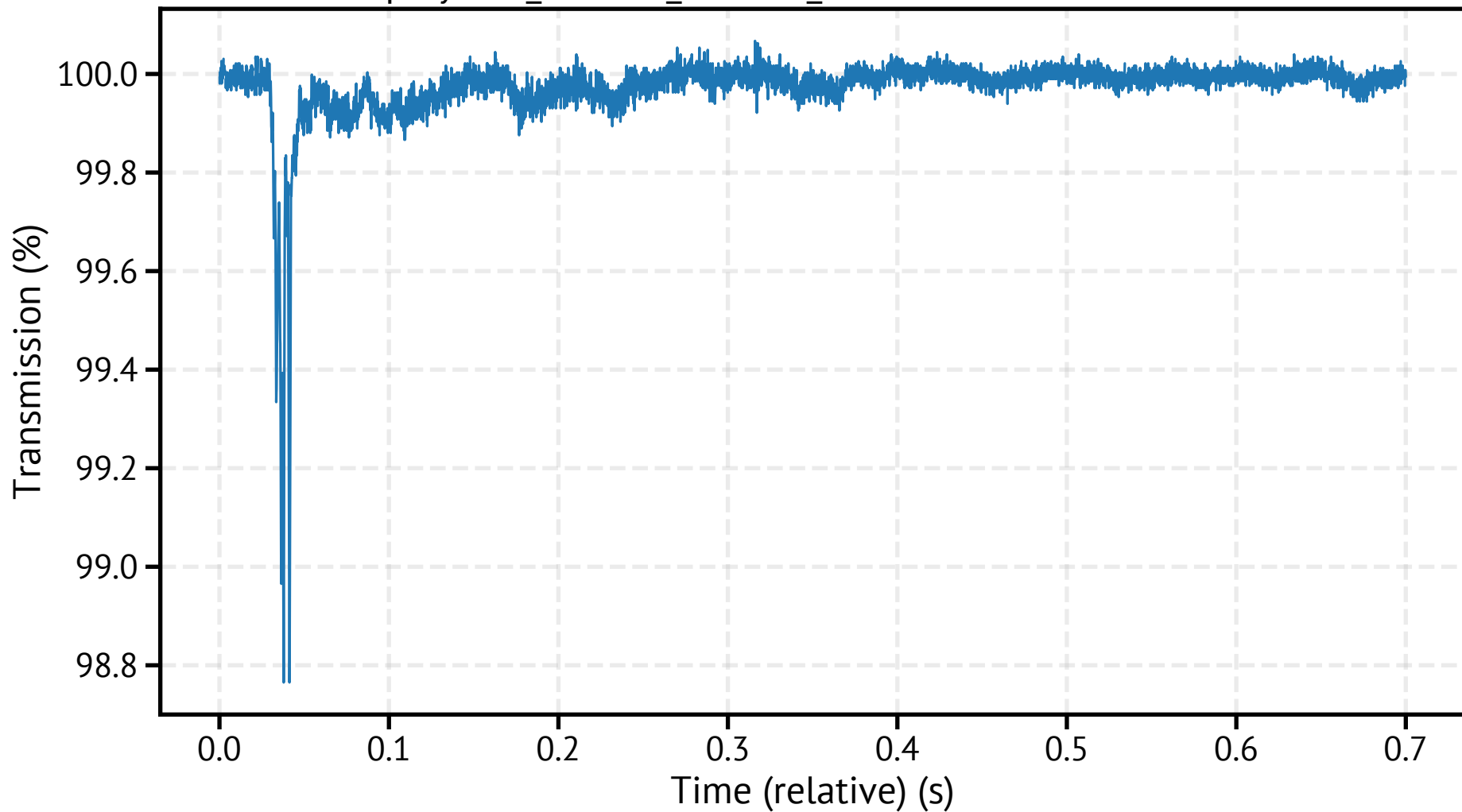
spraytec1_260318_120750_309000.csv - Transmission
