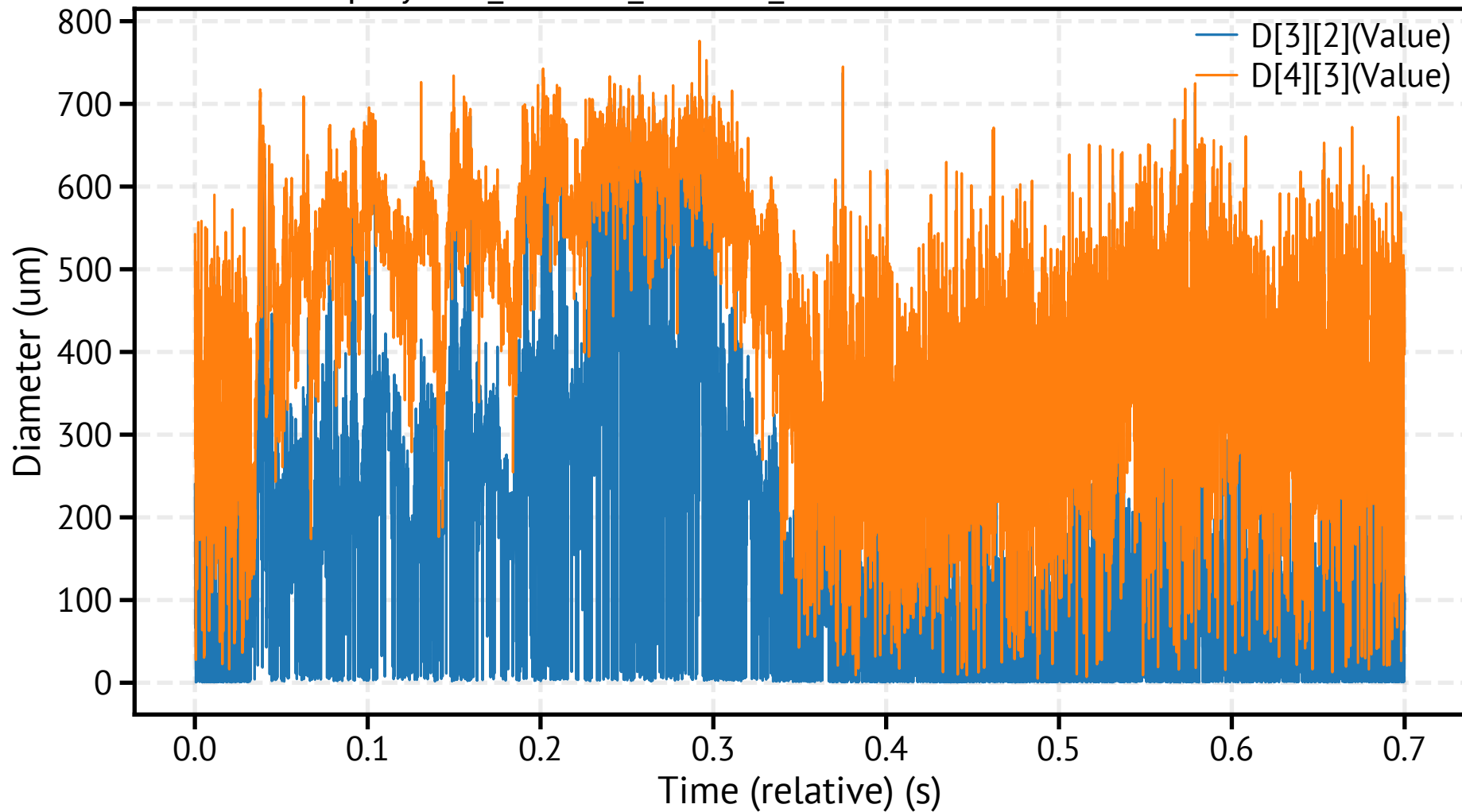
spraytec2_260318_120848_000900.csv - Mean Diameters
