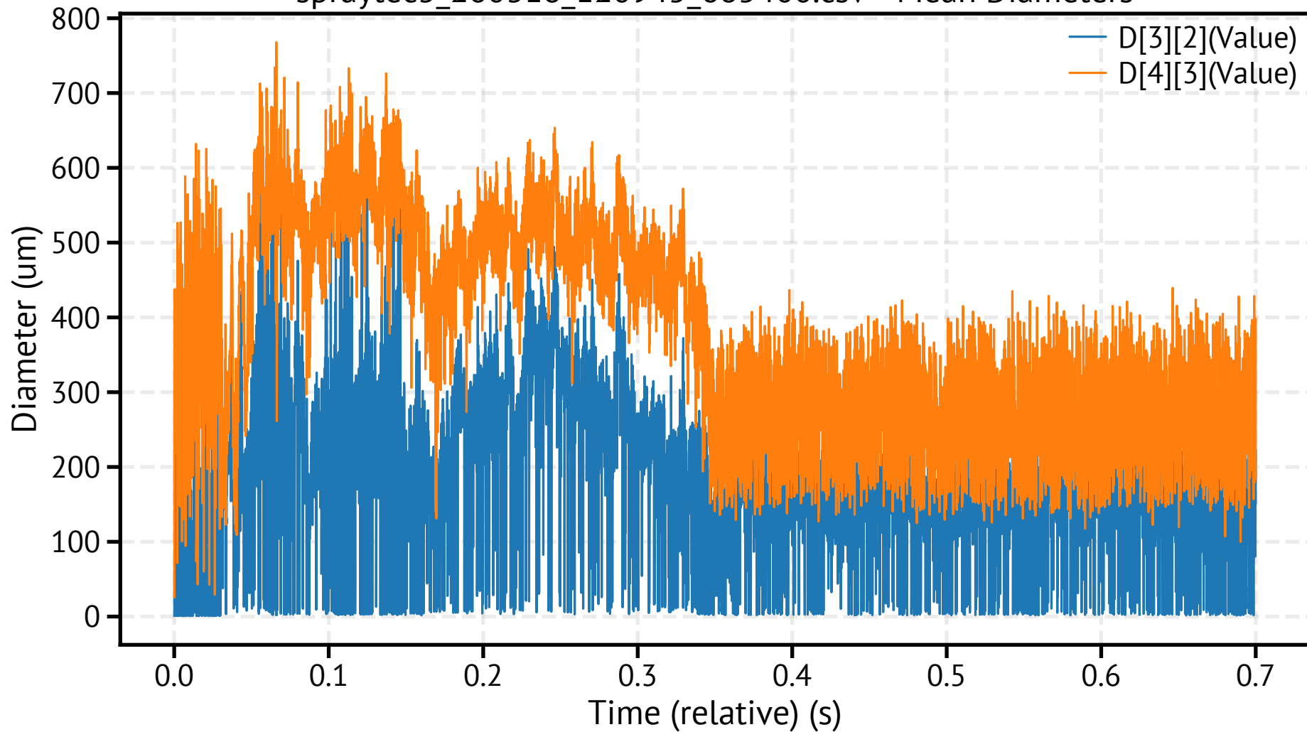
spraytec3_260318_120945_685400.csv - Mean Diameters
