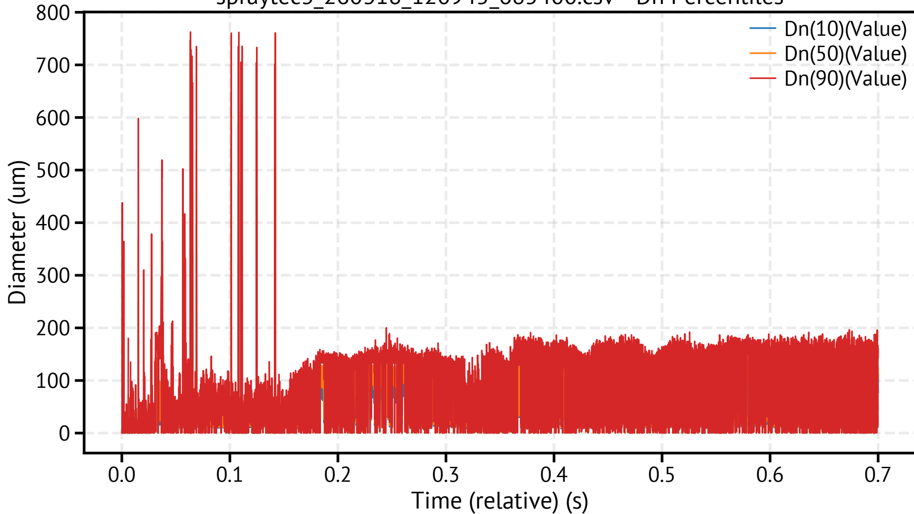
spraytec3_260318_120945_685400.csv - Dn Percentiles
