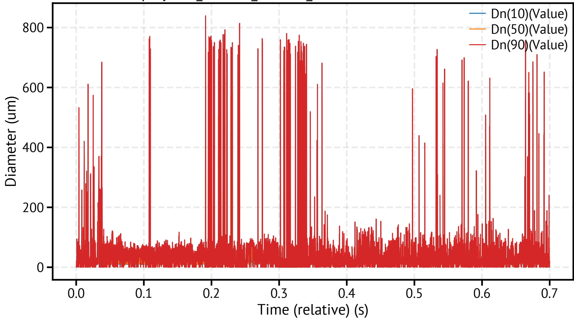
spraytec5_260318_121141_072000.csv - Dn Percentiles
