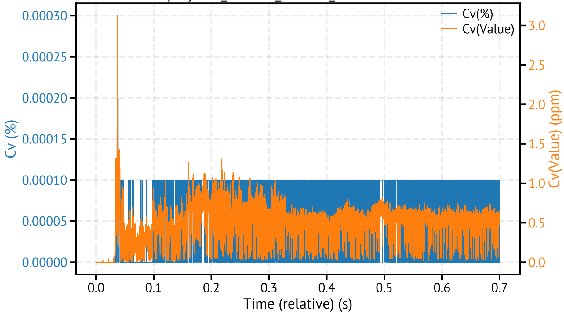
spraytec6_260318_121238_869200.csv - Cv
