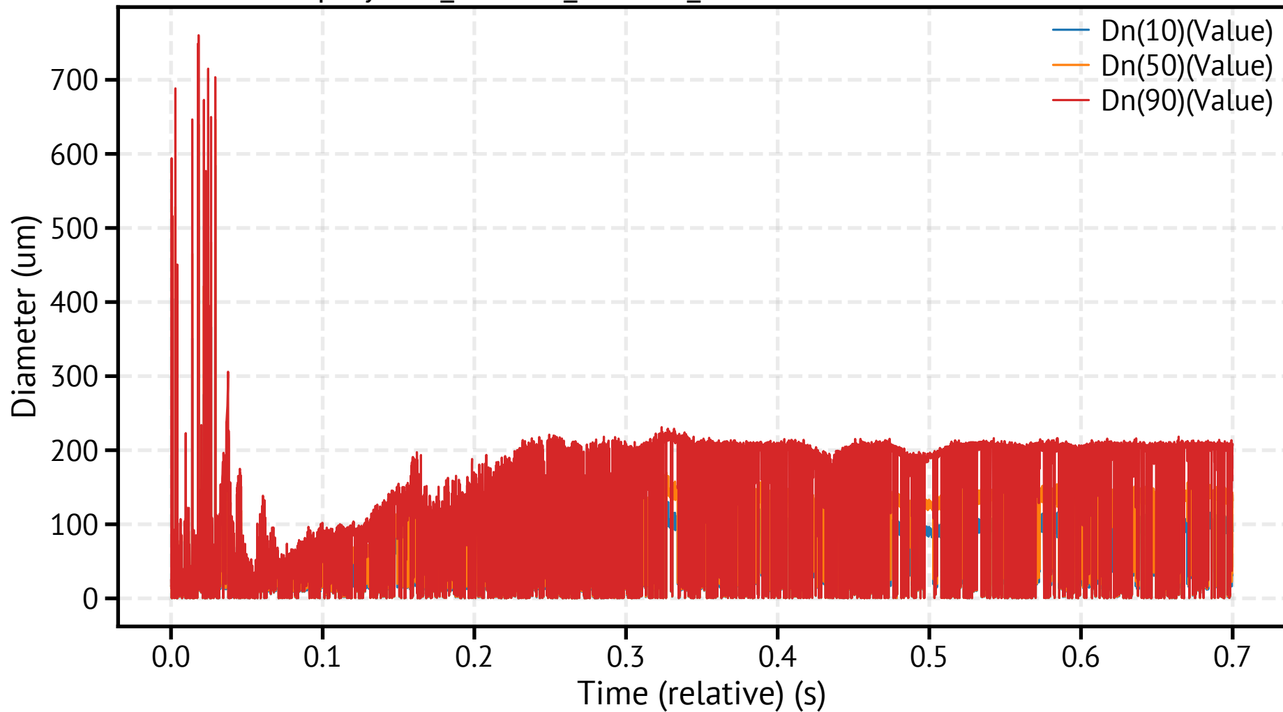
spraytec6_260318_121238_869200.csv - Dn Percentiles
