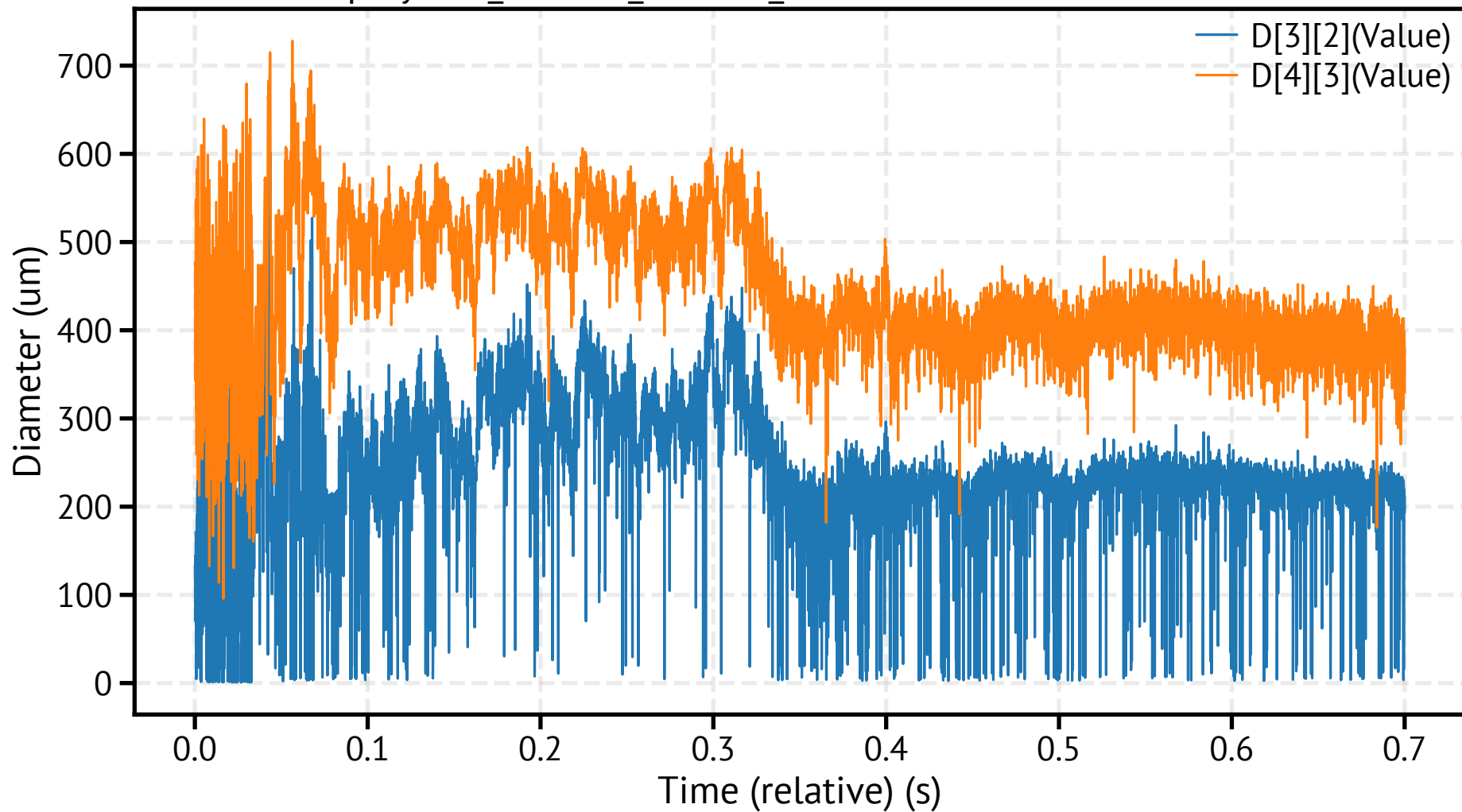
spraytec7_260318_121336_590200.csv - Mean Diameters
