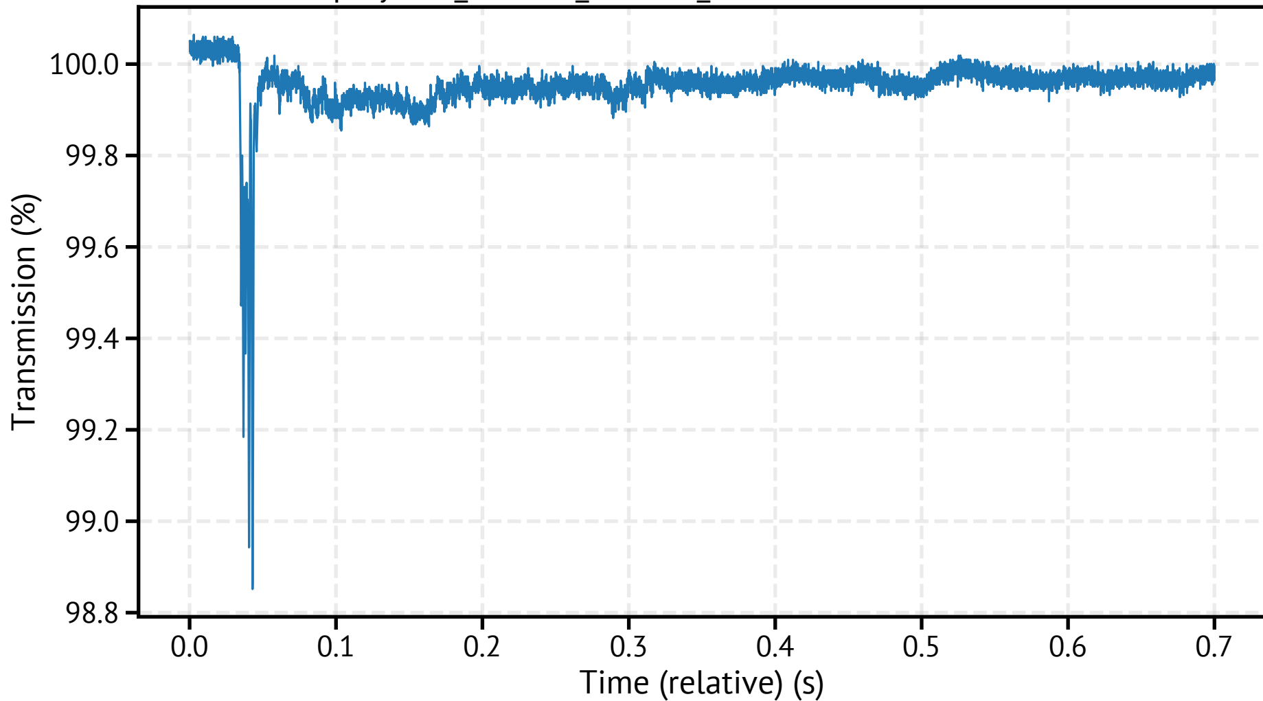
spraytec7_260318_121336_590200.csv - Transmission
