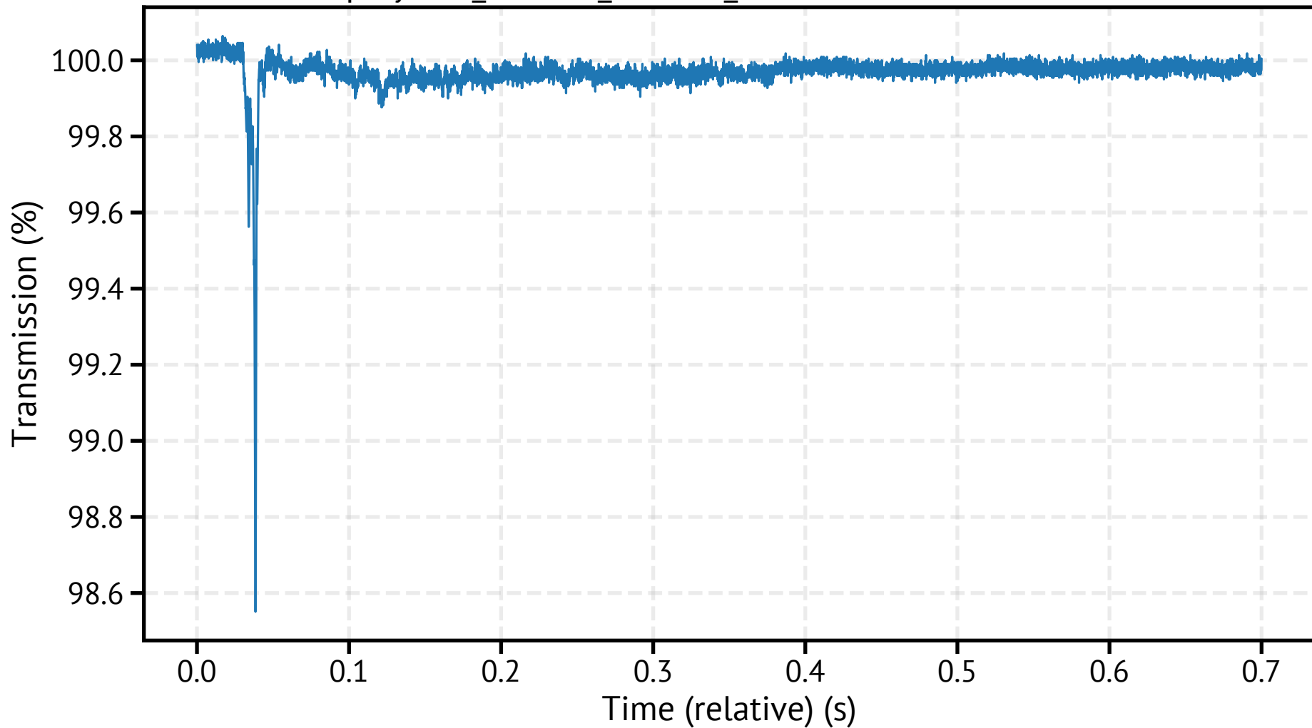
spraytec8_260318_121434_233900.csv - Transmission
