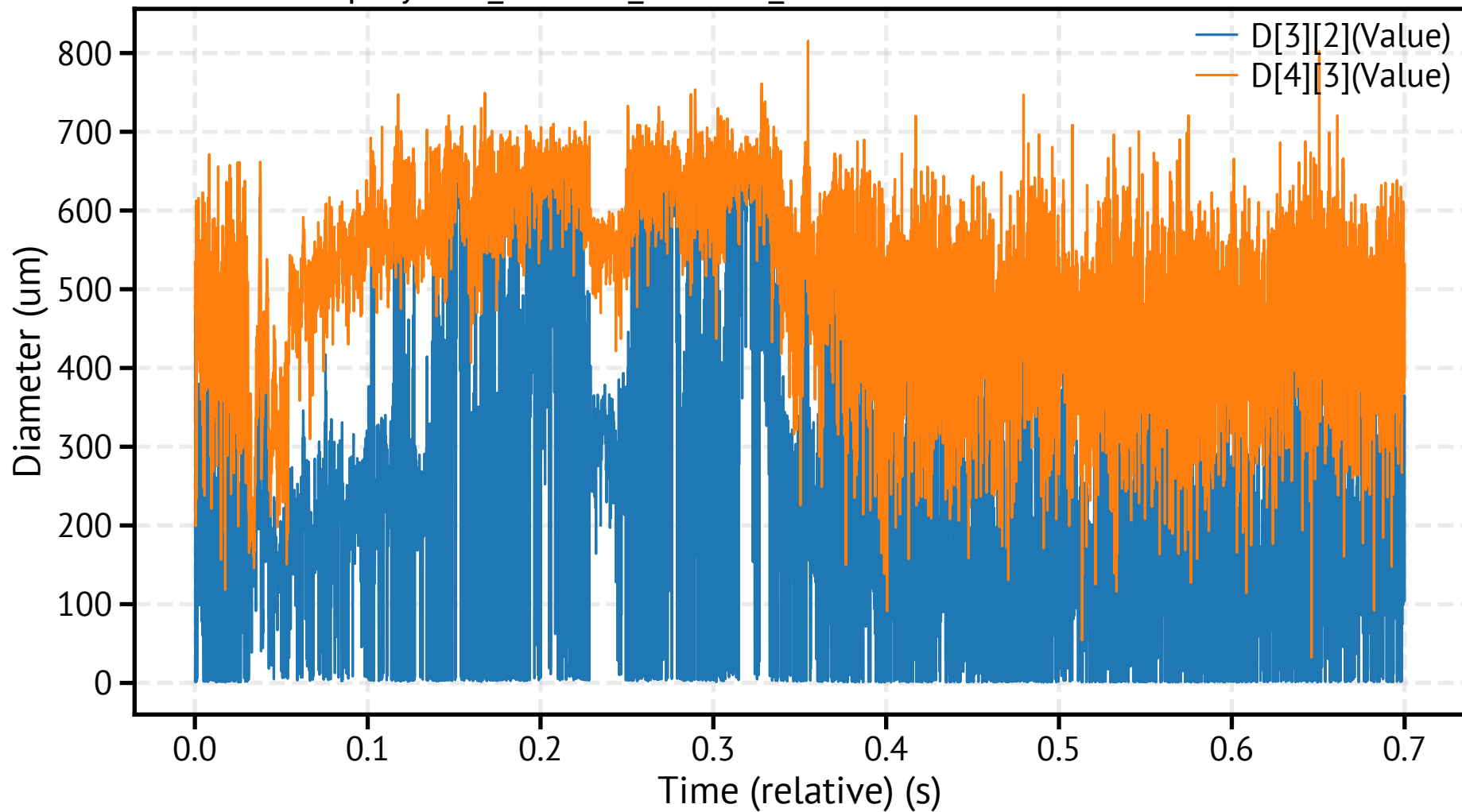
spraytec9_260318_121531_953800.csv - Mean Diameters
