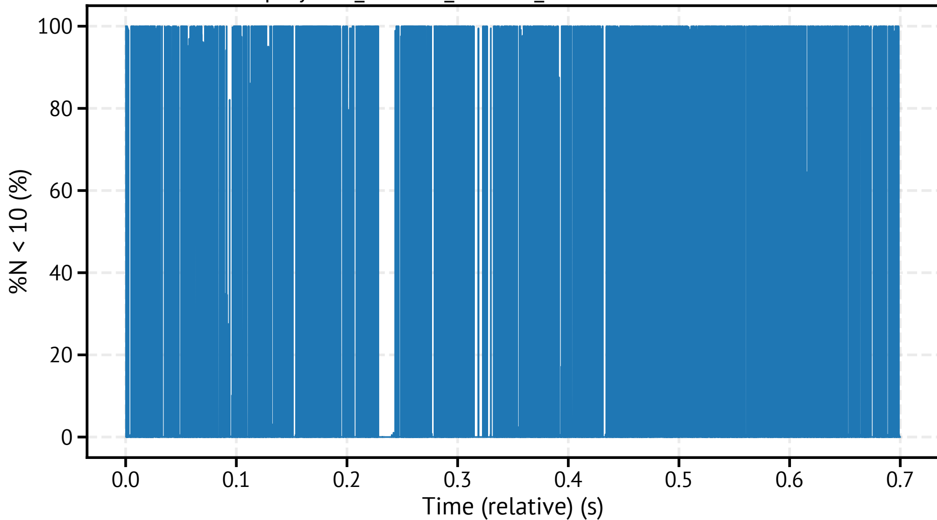
spraytec9_260318_121531_953800.csv - %N < 10
