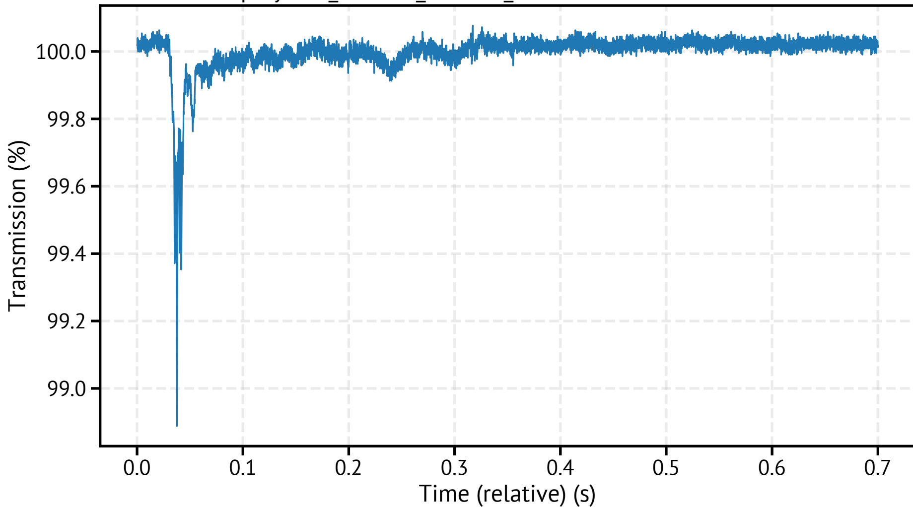
spraytec9_260318_121531_953800.csv - Transmission
