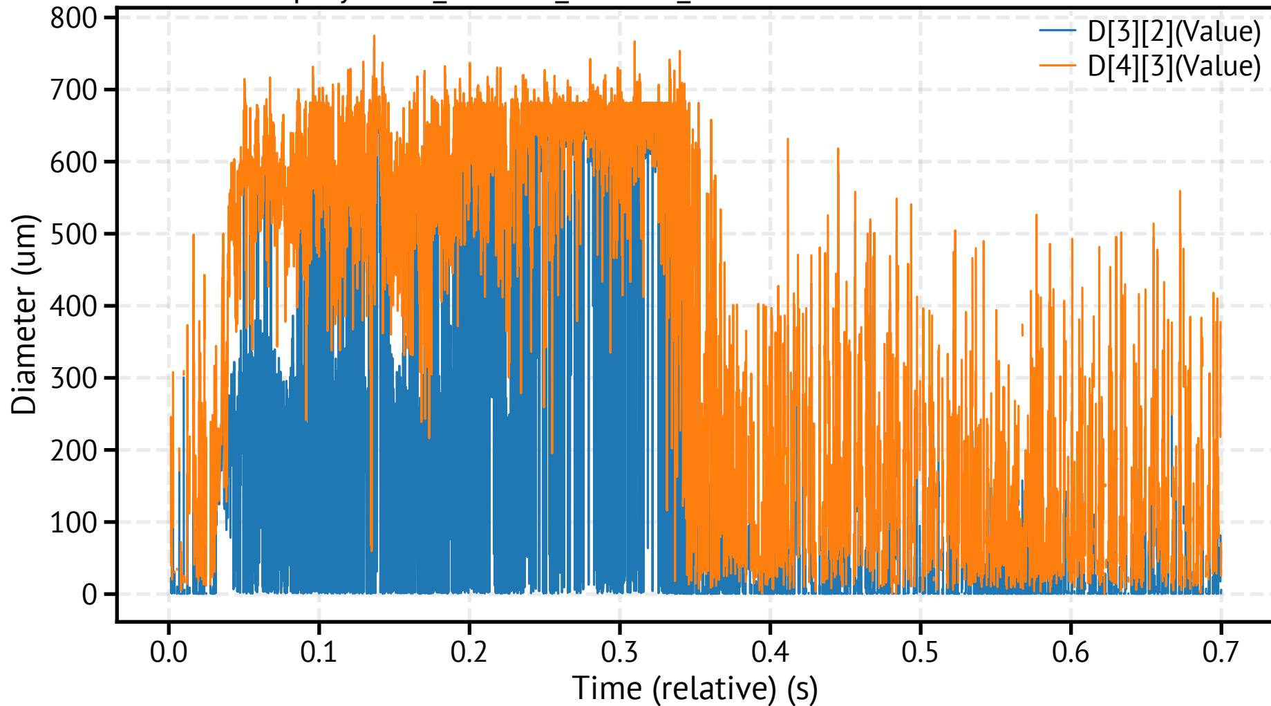
spraytec10_260318_123004_342300.csv - Mean Diameters
