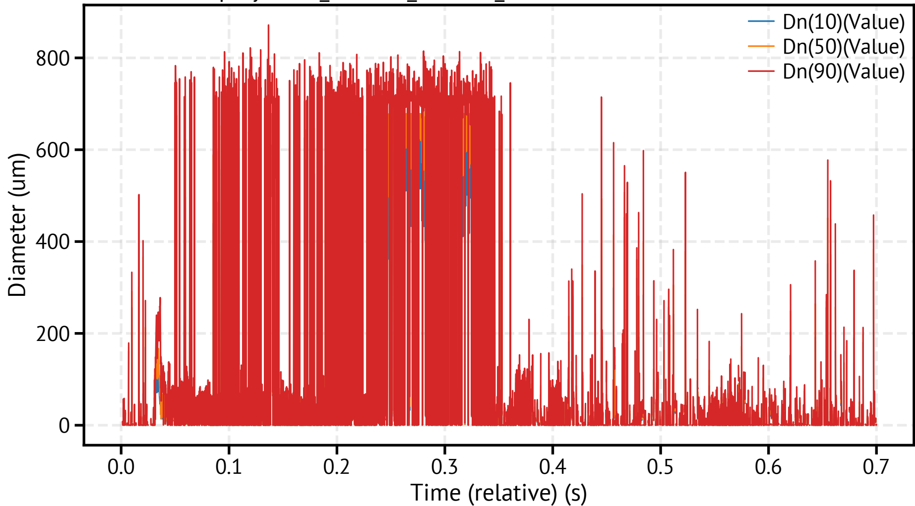
spraytec10_260318_123004_342300.csv - Dn Percentiles
