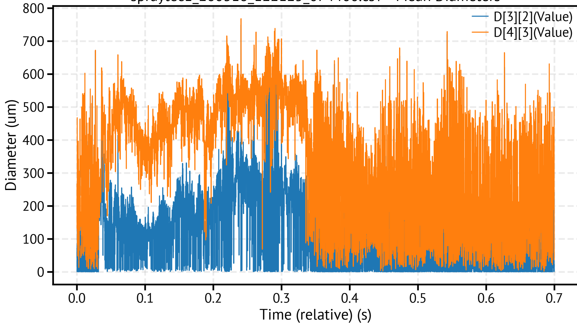
spraytec1_260318_122125_074400.csv - Mean Diameters
