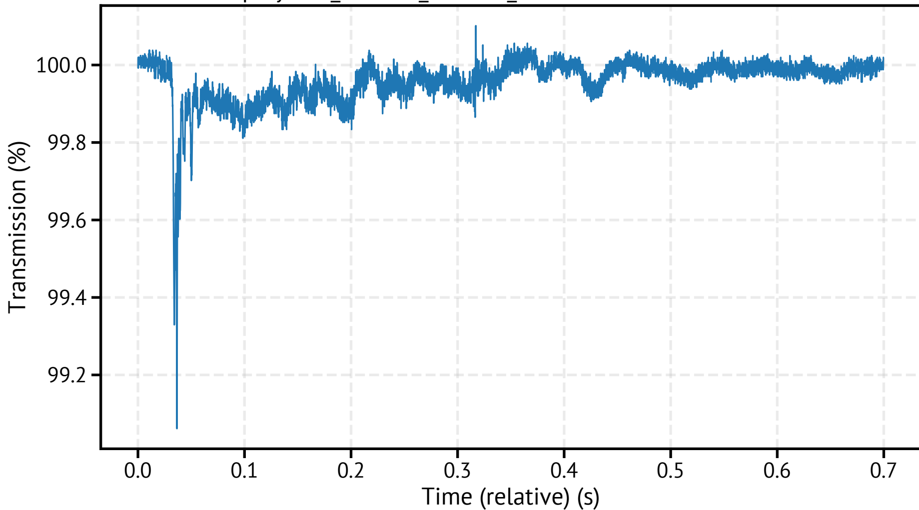
spraytec1_260318_122125_074400.csv - Transmission
