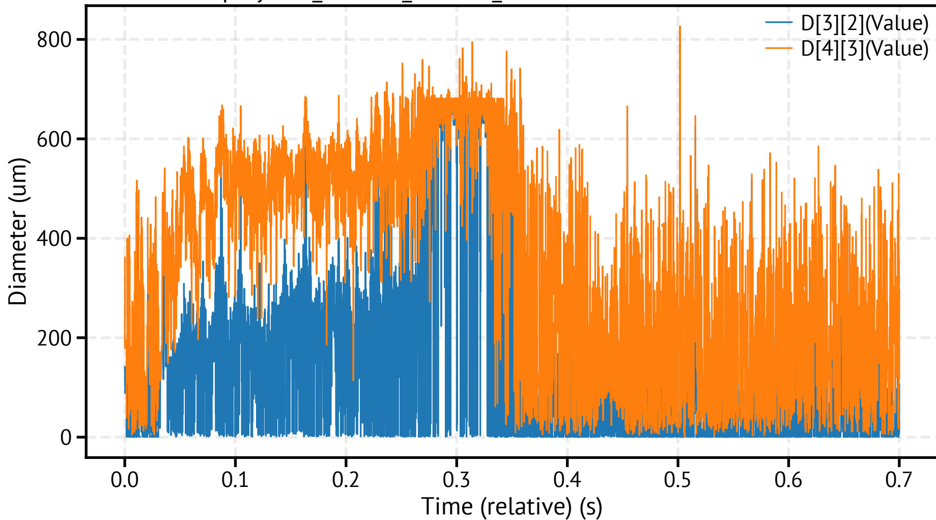
spraytec3_260318_122320_395100.csv - Mean Diameters
