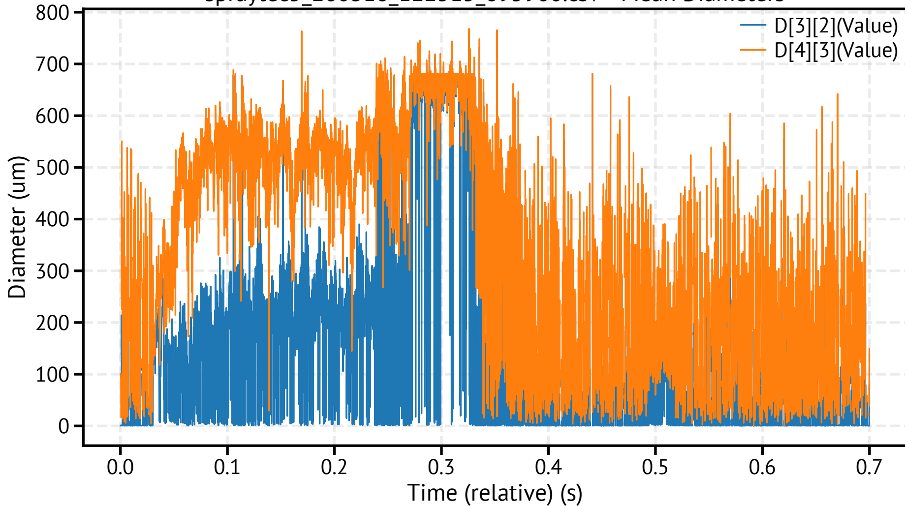
spraytec5_260318_122515_895900.csv - Mean Diameters
