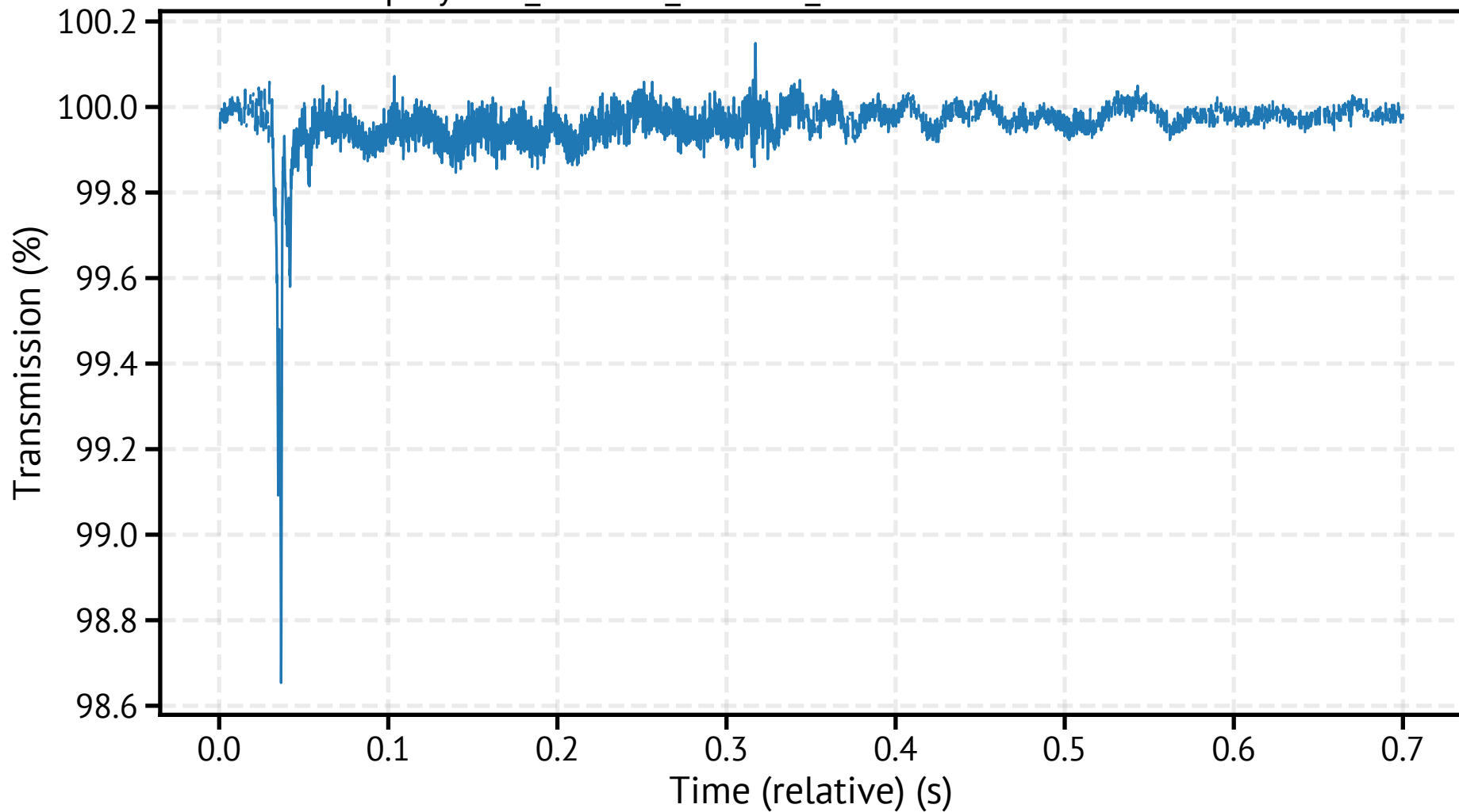
spraytec6_260318_122613_478600.csv - Transmission
