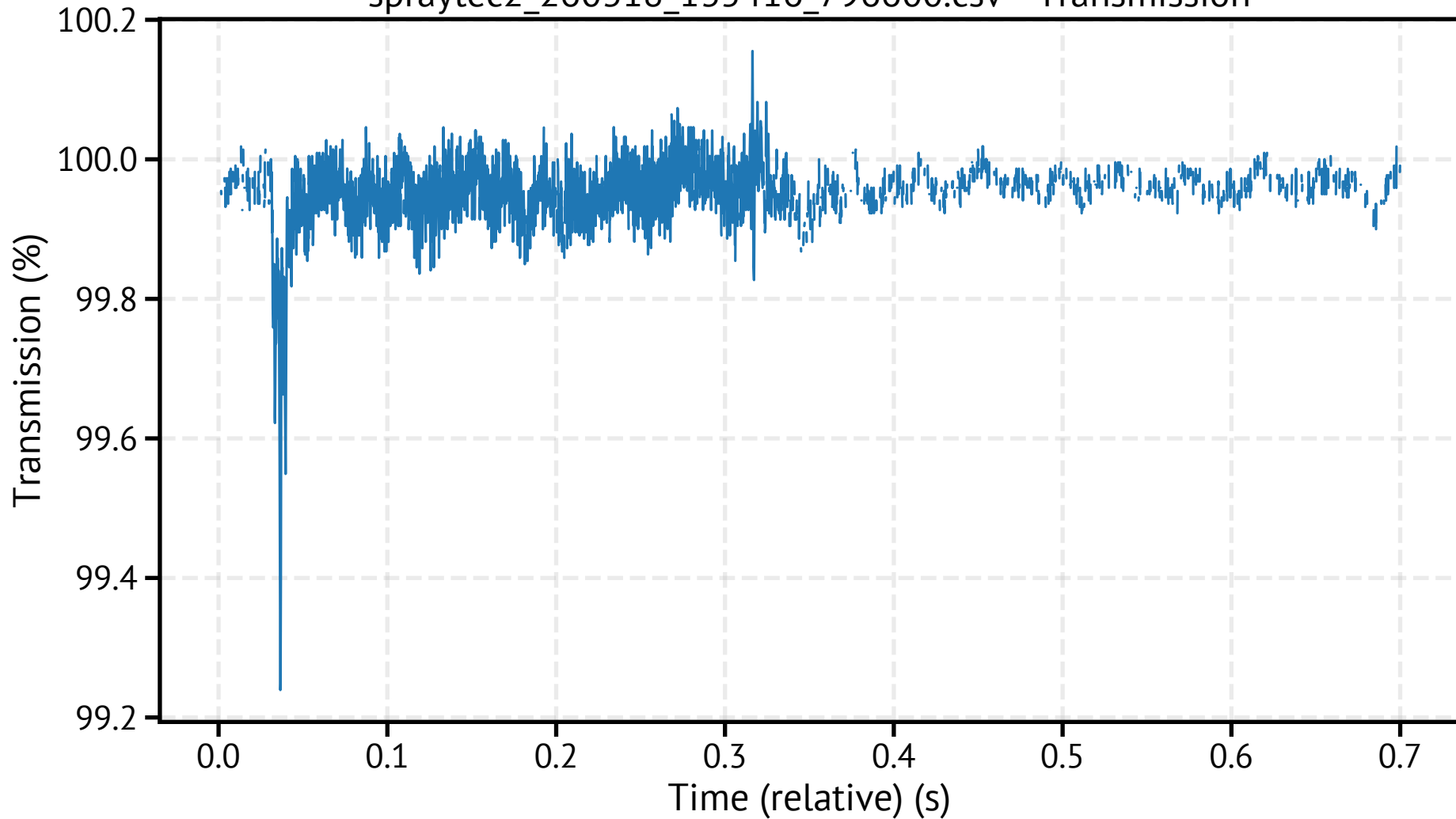
spraytec2_260318_135416_796600.csv - Transmission
