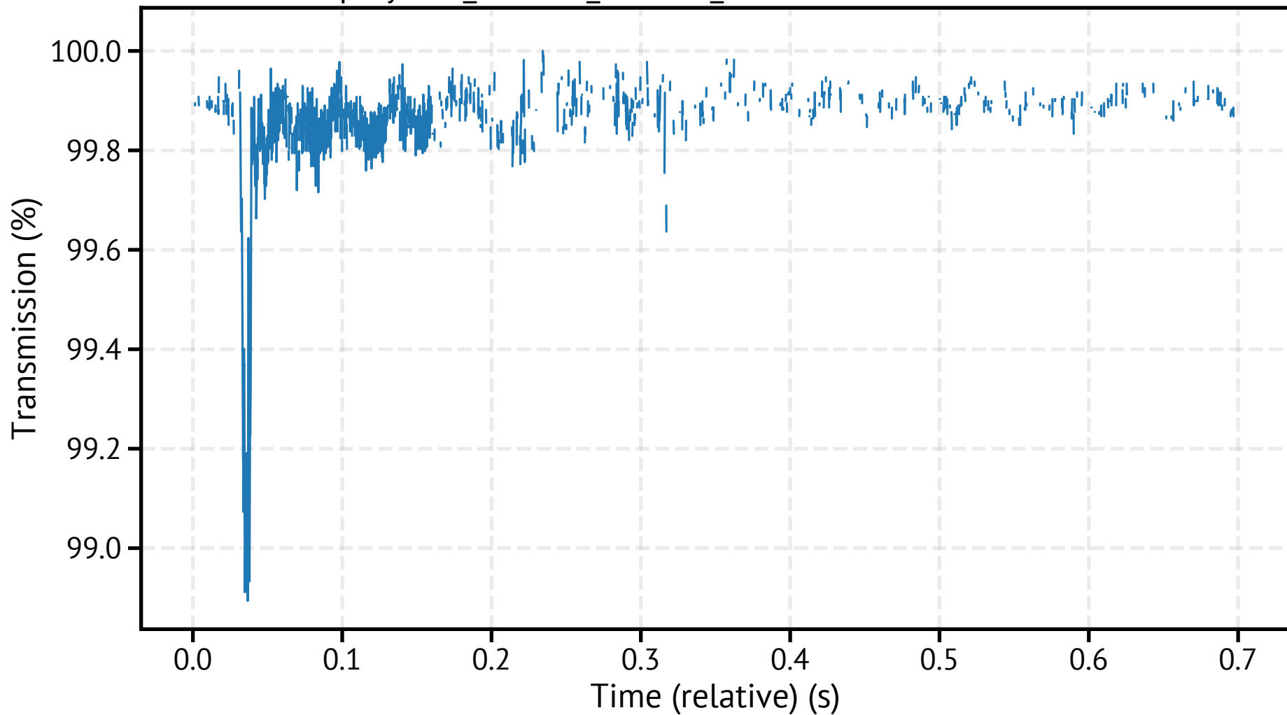
spraytec6_260318_135807_459300.csv - Transmission
