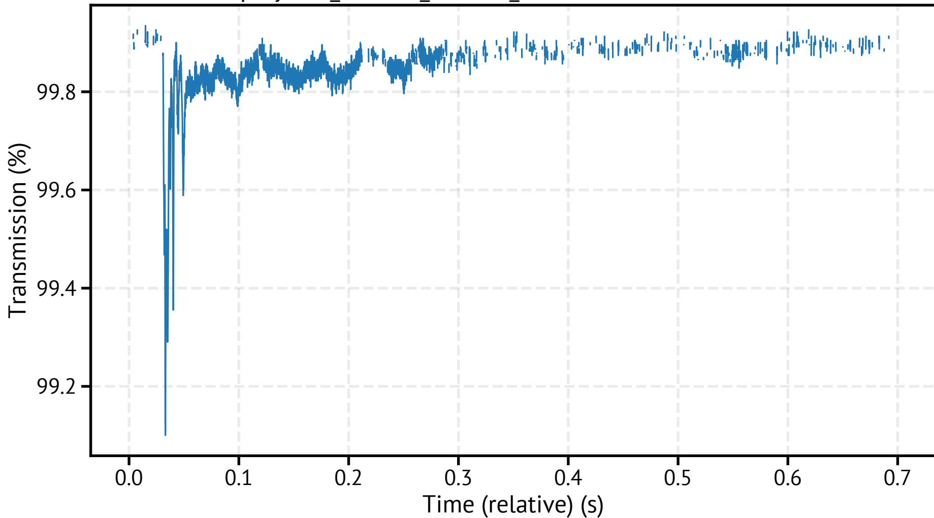
spraytec9_260318_140100_404400.csv - Transmission
