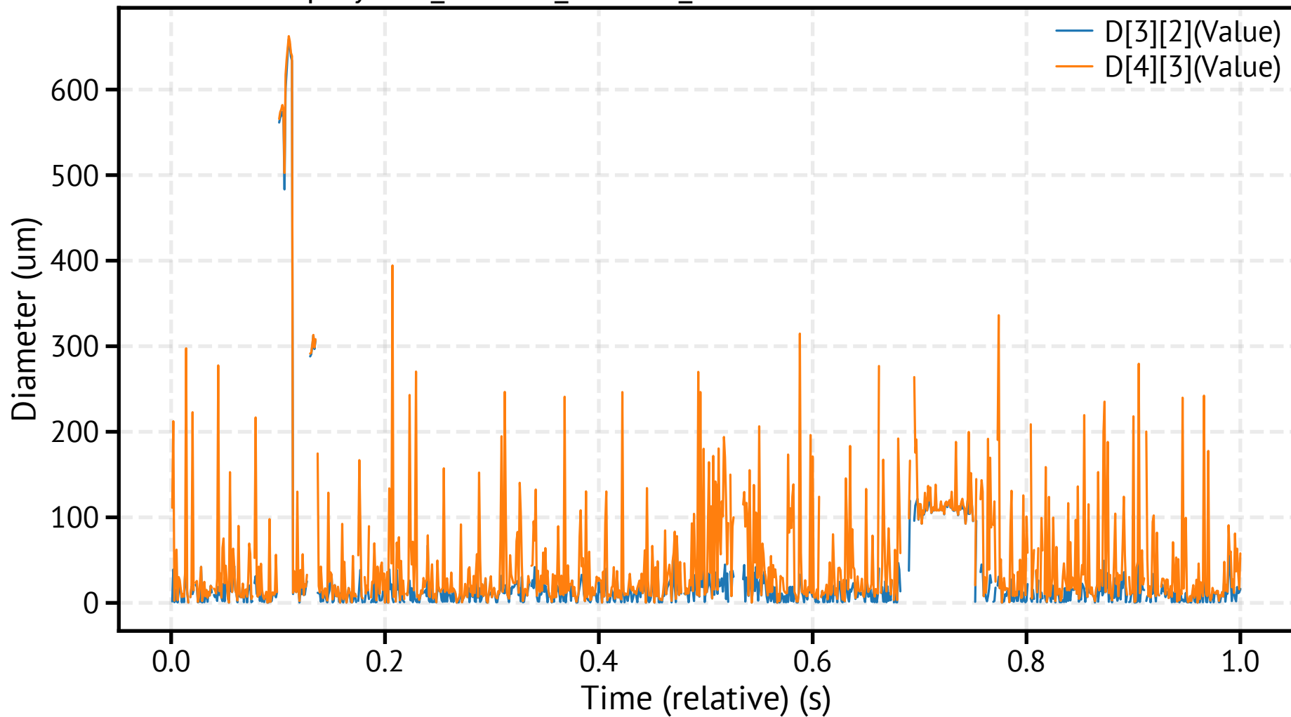
spraytec1_260304_115013_741600.csv - Mean Diameters
