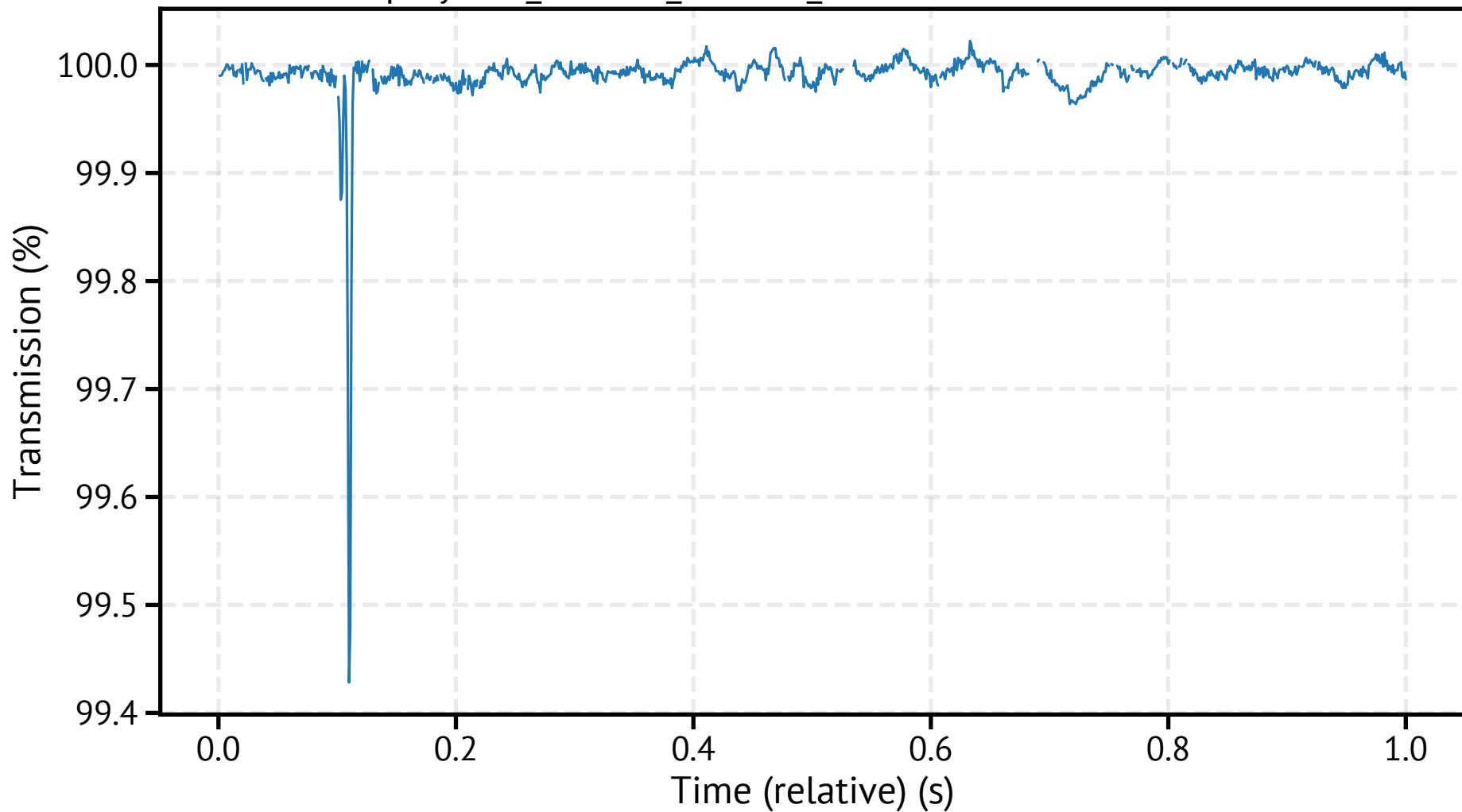
spraytec1_260304_115013_741600.csv - Transmission
