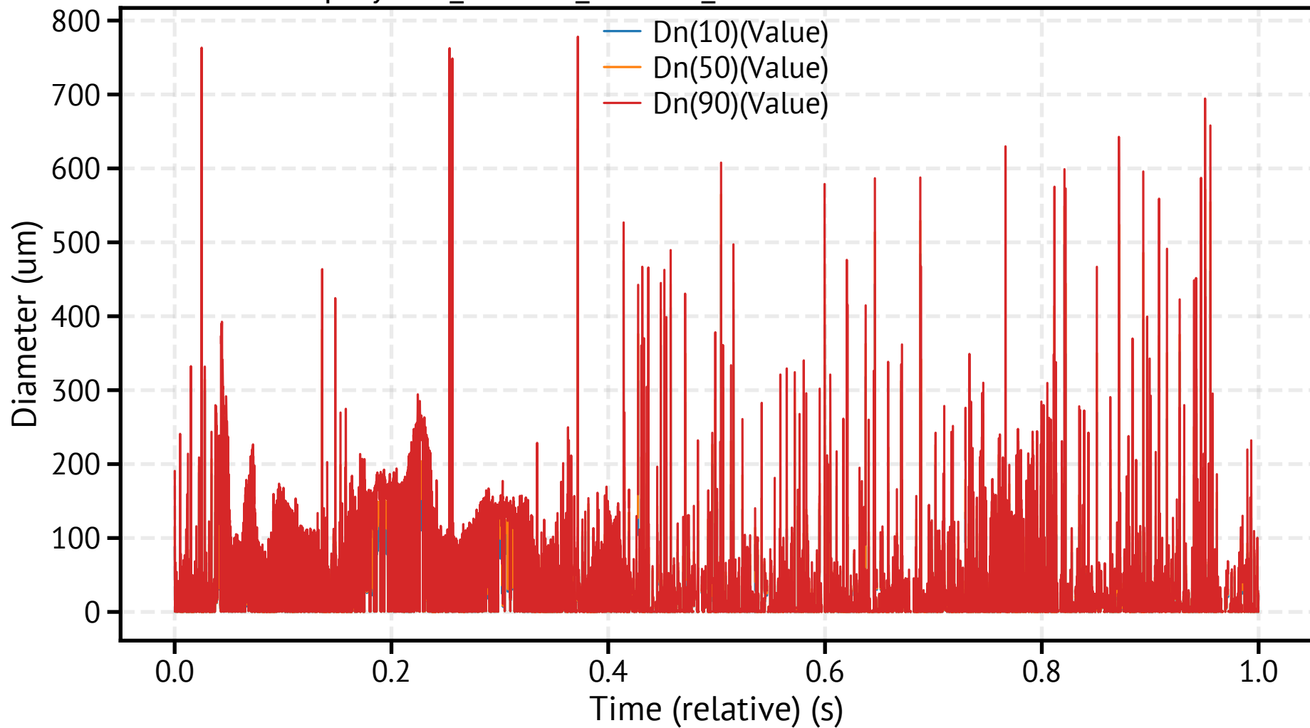
spraytec1_260310_133402_766800.csv - Dn Percentiles
