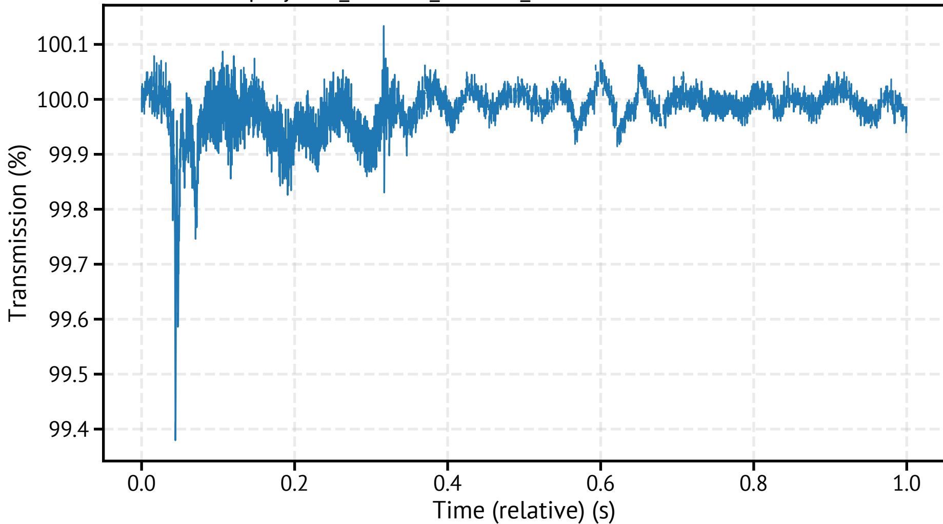
spraytec1_260310_133402_766800.csv - Transmission
