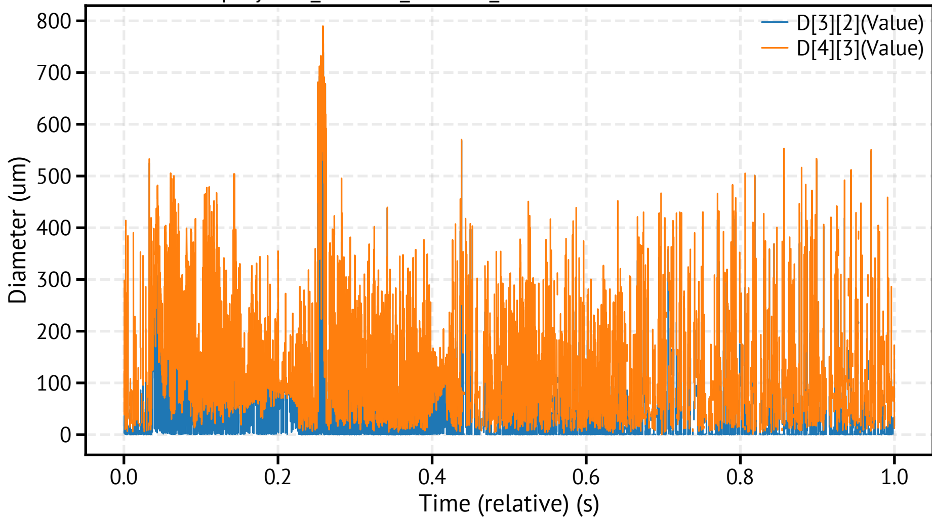
spraytec2_260310_133430_575700.csv - Mean Diameters
