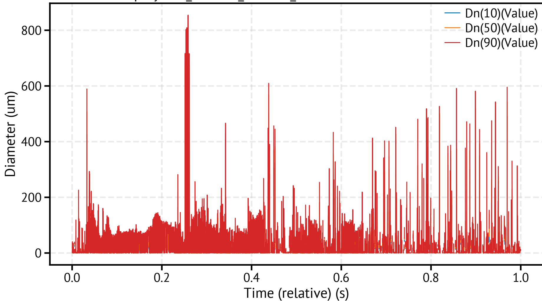
spraytec2_260310_133430_575700.csv - Dn Percentiles
