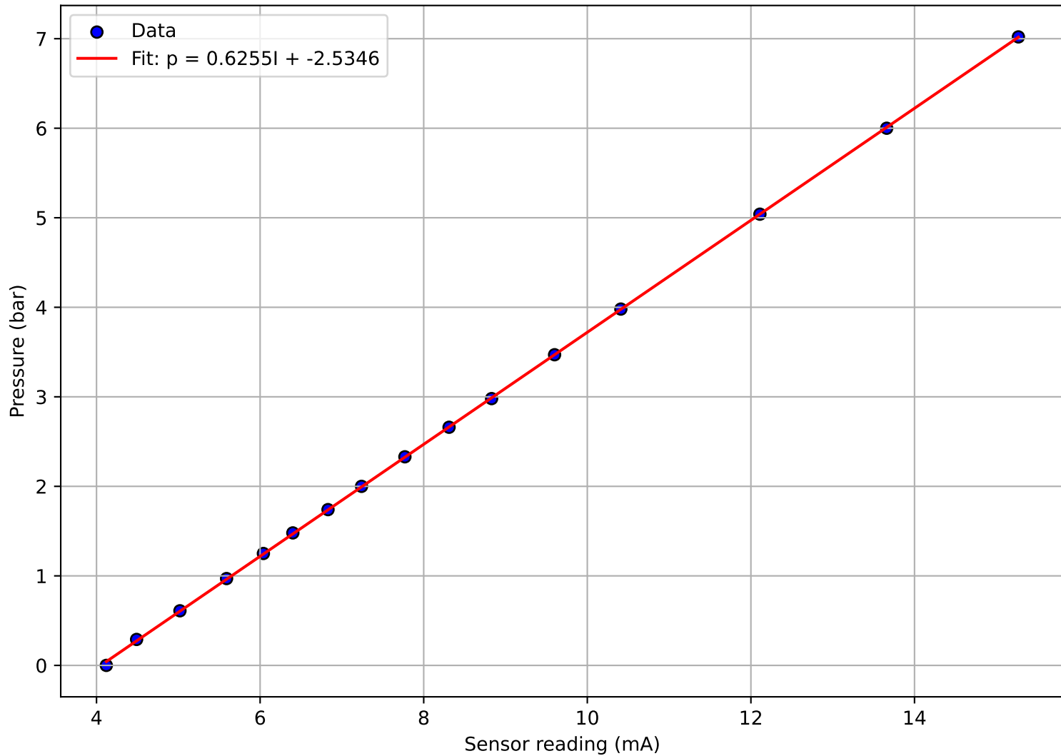
Pressure sensor calibration - Rclick_calibration_new2
