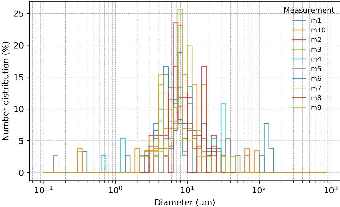
Series 8 (Morgan) PEO600k 0.5%
