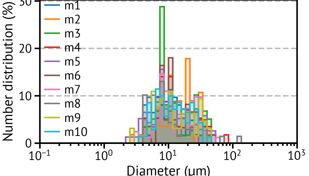
Series 6 (Morgan) PEO600k 0.1%
