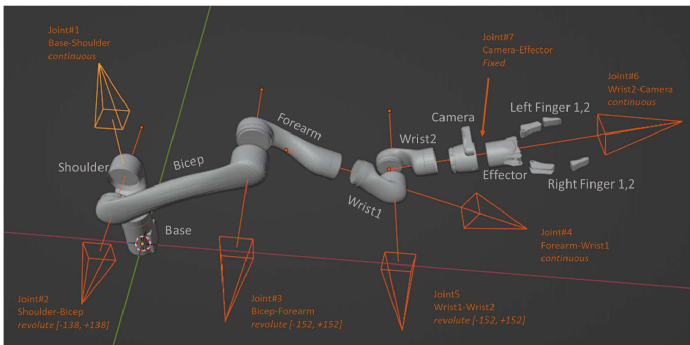
Figure 6. Robotic Arm with Links and Joints.
