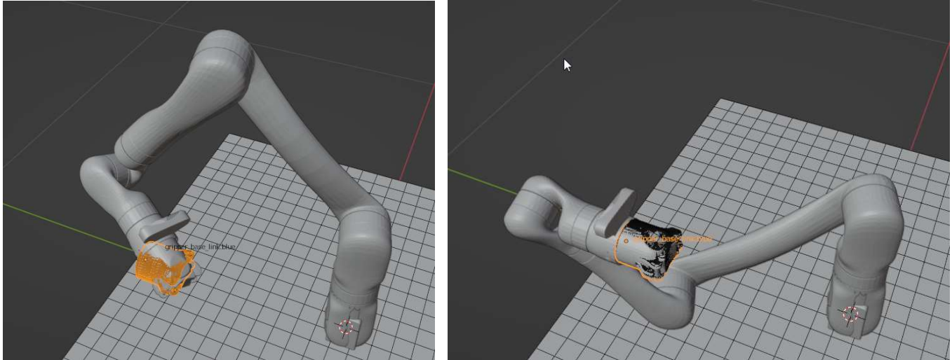
Figure 19. IK Problem, impact of the Local Minimum
