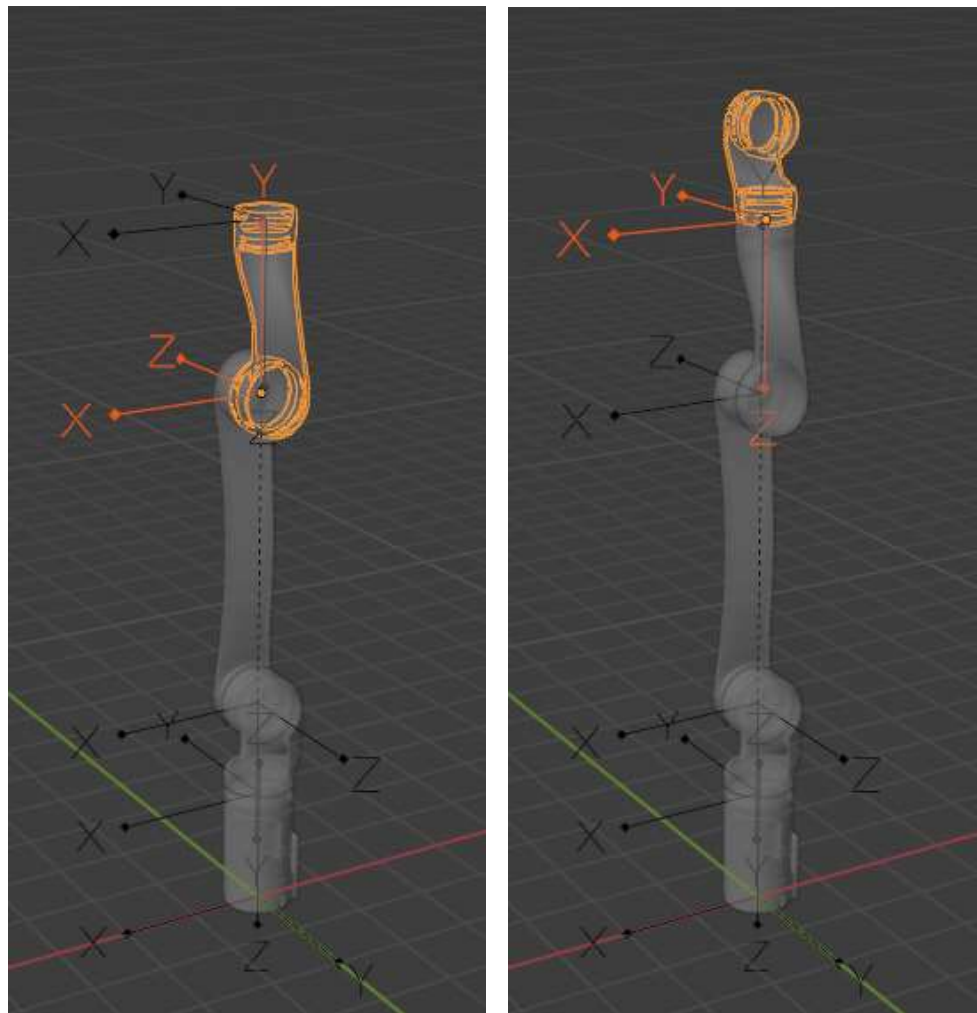
Figure 10. 4 th Link Composition.
