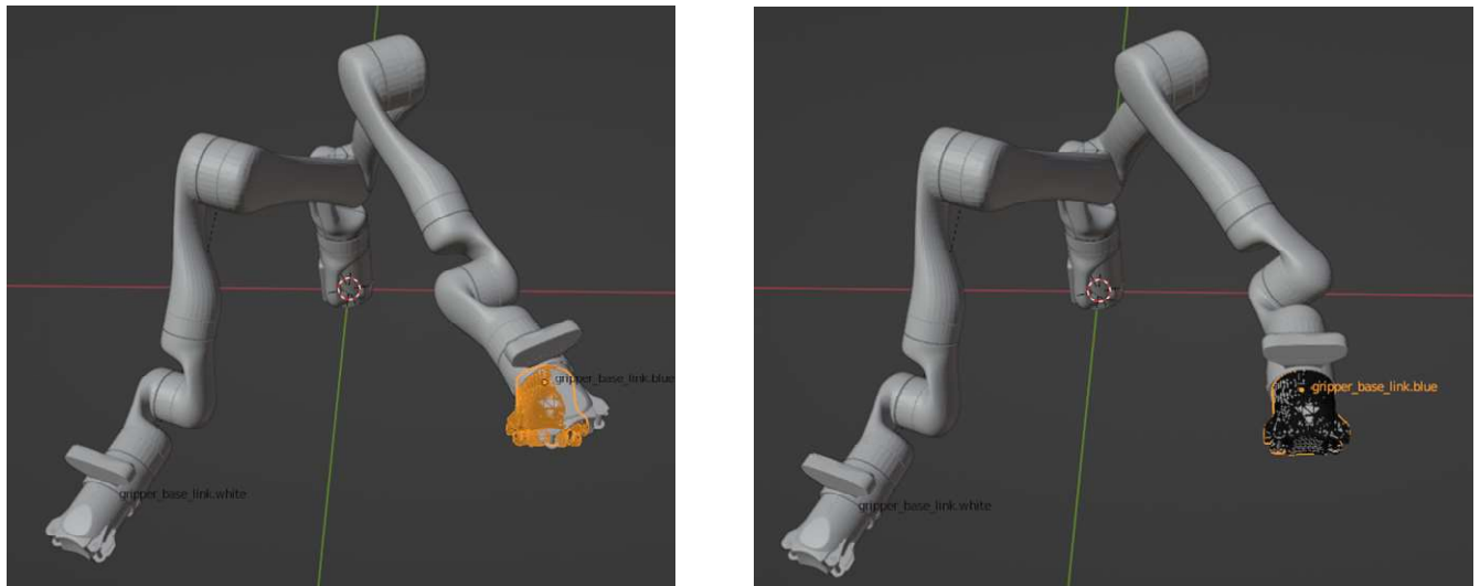
Figure 17. Incorrect and Correct Solution of the IK Problem.
