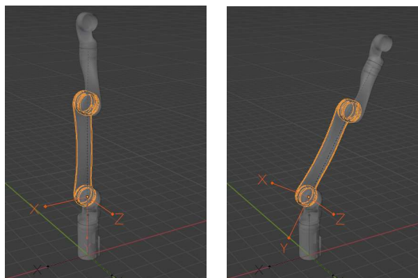
Figure 12. Link Composition with Joint Angle.
