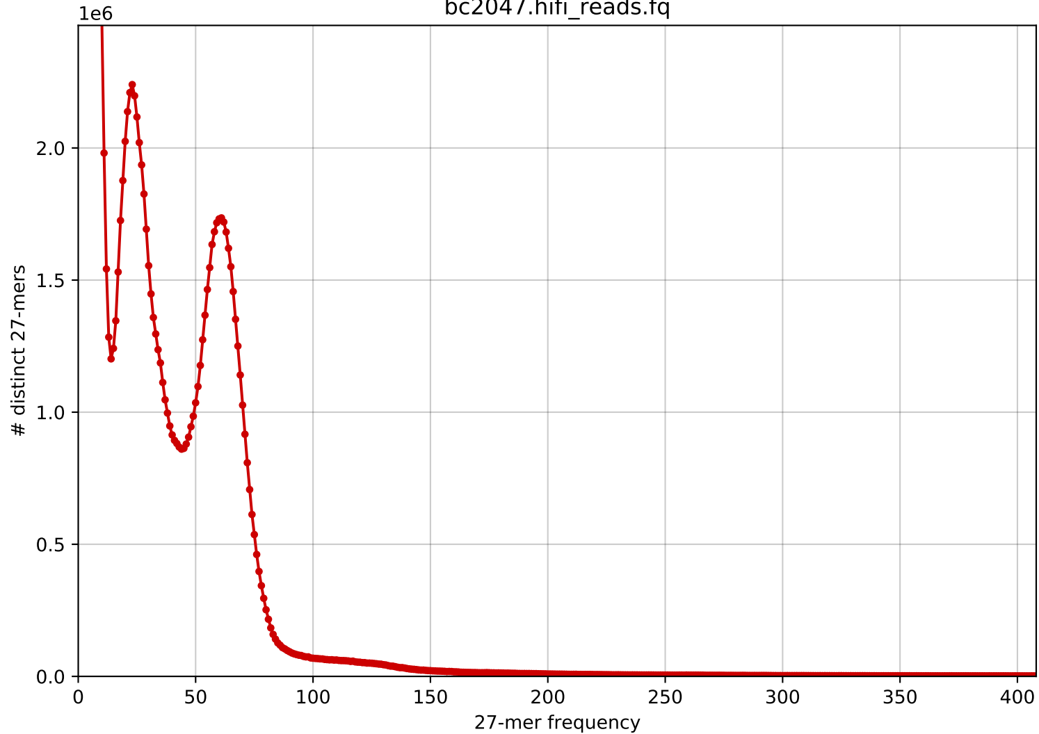
27-mer spectra for: m64041_230527_063349.bc2047-- bc2047.hifi_reads.fq
