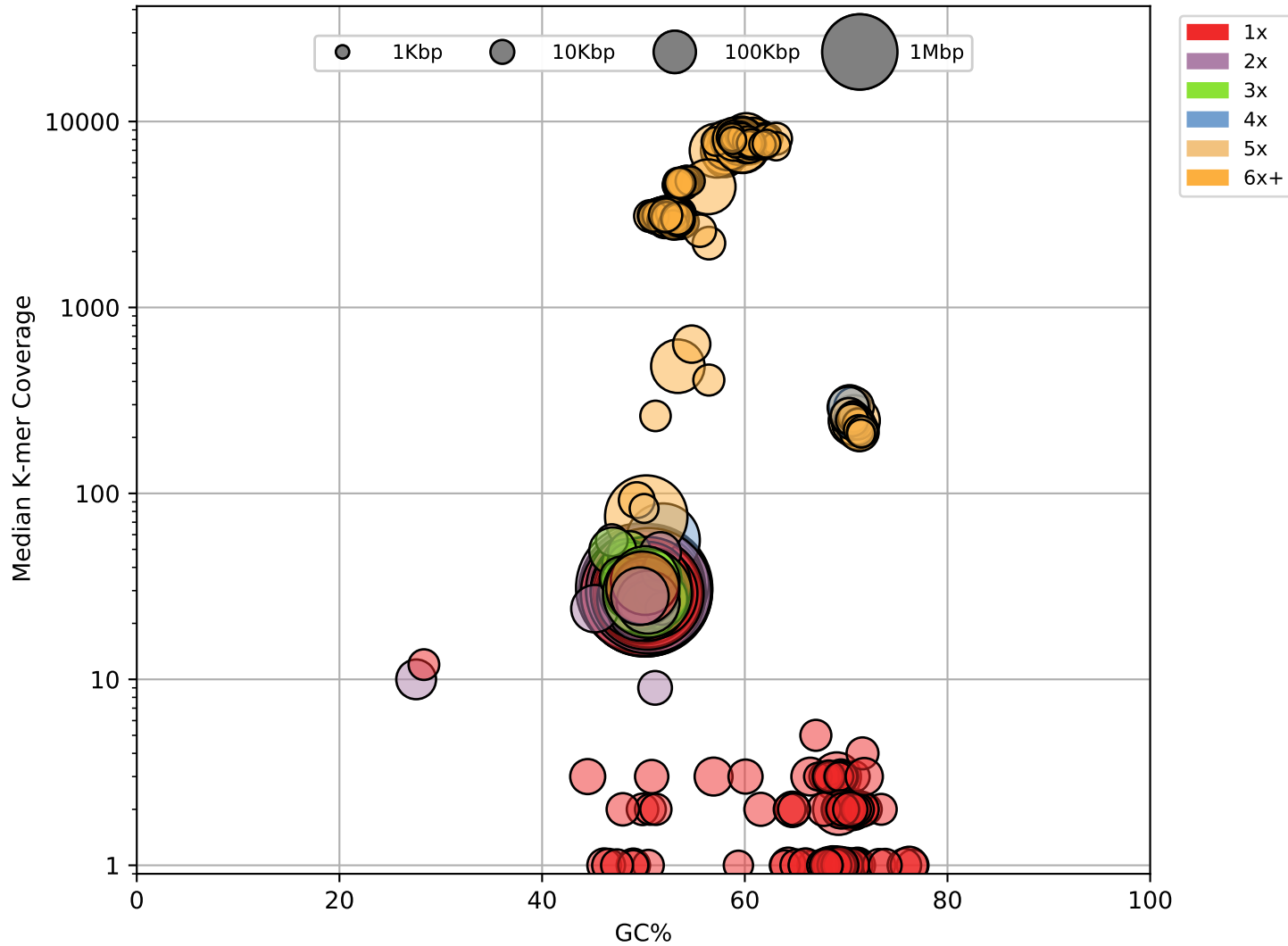
KAT Contig Length and Duplication plot
